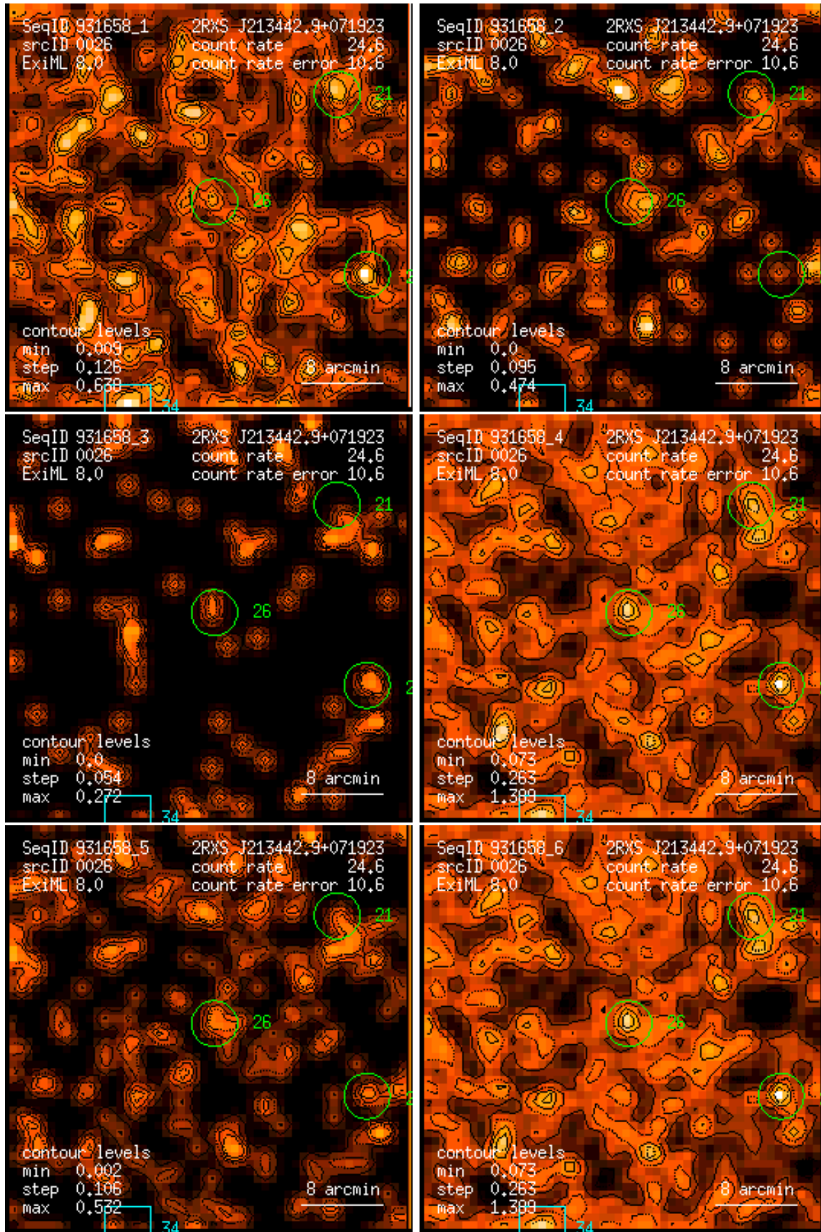
Figure 26: RASS 931658: detection 0026: band rate images, Gaussian filter: (1) PSPC channels 11 – 41, (2) 52 – 90, (3) 91 – 201, (4) 11 – 235, (5) 52 – 201, (6) 11 – 201. Broad band rates in counts/ks. Band rate contour levels in counts/ks/arcmin 2 .
