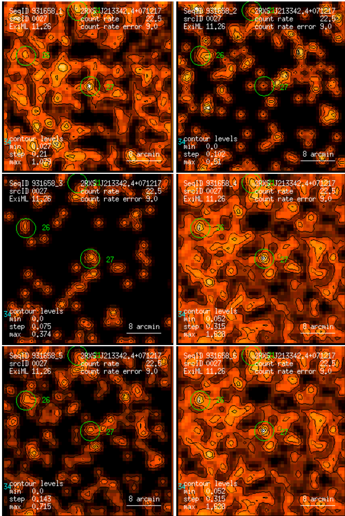
Figure 27: RASS 931658: detection 0027: band rate images, Gaussian filter: (1) PSPC channels 11 – 41, (2) 52 – 90, (3) 91 – 201, (4) 11 – 235, (5) 52 – 201, (6) 11 – 201. Broad band rates in counts/ks. Band rate contour levels in counts/ks/arcmin 2 .
