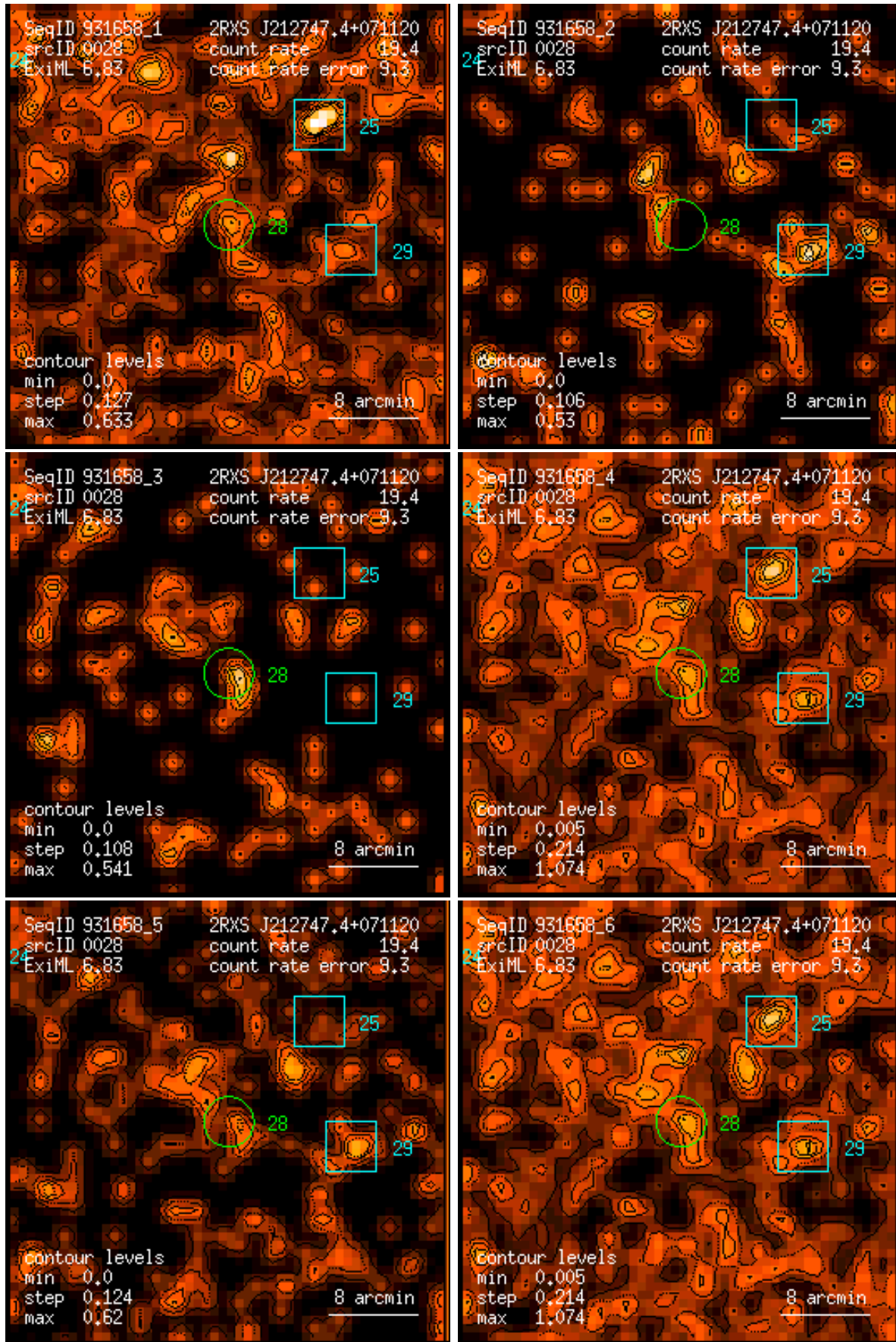
Figure 28: RASS 931658: detection 0028: band rate images, Gaussian filter: (1) PSPC channels 11 – 41, (2) 52 – 90, (3) 91 – 201, (4) 11 – 235, (5) 52 – 201, (6) 11 – 201. Broad band rates in counts/ks. Band rate contour levels in counts/ks/arcmin 2 .
