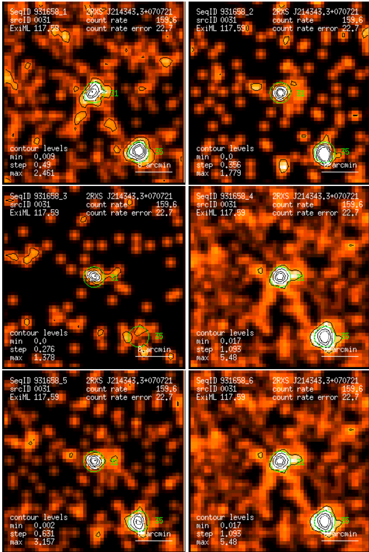
Figure 31: RASS 931658: detection 0031: band rate images, Gaussian filter: (1) PSPC channels 11 – 41, (2) 52 – 90, (3) 91 – 201, (4) 11 – 235, (5) 52 – 201, (6) 11 – 201. Broad band rates in counts/ks. Band rate contour levels in counts/ks/arcmin 2 .
