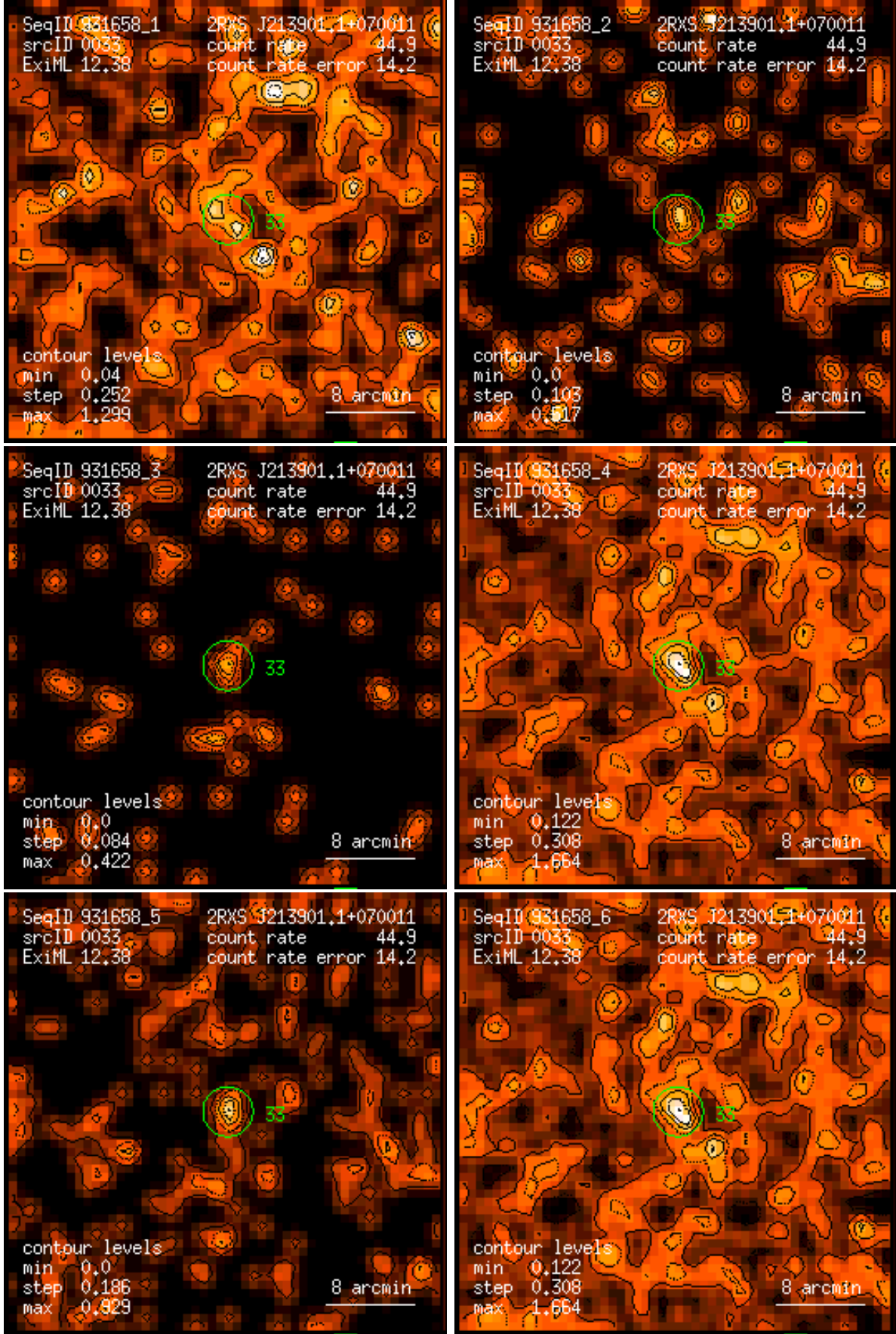
Figure 33: RASS 931658: detection 0033: band rate images, Gaussian filter: (1) PSPC channels 11 – 41, (2) 52 – 90, (3) 91 – 201, (4) 11 – 235, (5) 52 – 201, (6) 11 – 201. Broad band rates in counts/ks. Band rate contour levels in counts/ks/arcmin 2 .
