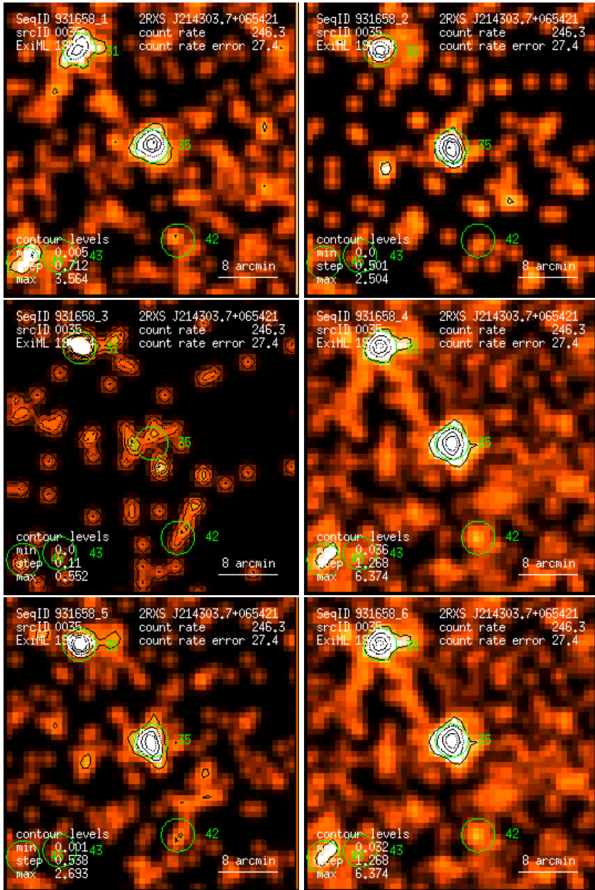
Figure 35: RASS 931658: detection 0035: band rate images, Gaussian filter: (1) PSPC channels 11 – 41, (2) 52 – 90, (3) 91 – 201, (4) 11 – 235, (5) 52 – 201, (6) 11 – 201. Broad band rates in counts/ks. Band rate contour levels in counts/ks/arcmin 2 .
