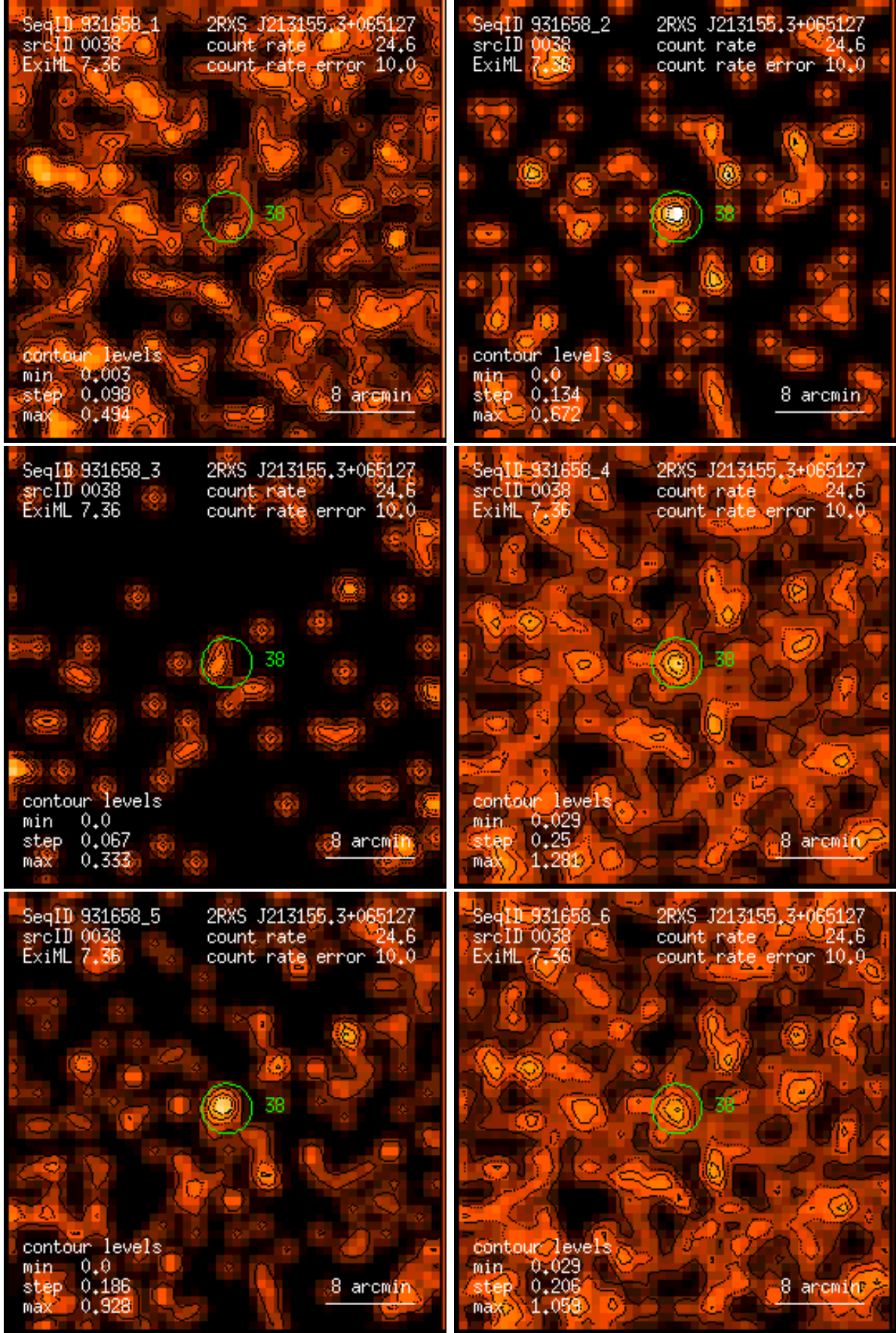
Figure 38: RASS 931658: detection 0038: band rate images, Gaussian filter: (1) PSPC channels 11 – 41, (2) 52 – 90, (3) 91 – 201, (4) 11 – 235, (5) 52 – 201, (6) 11 – 201. Broad band rates in counts/ks. Band rate contour levels in counts/ks/arcmin 2 .
