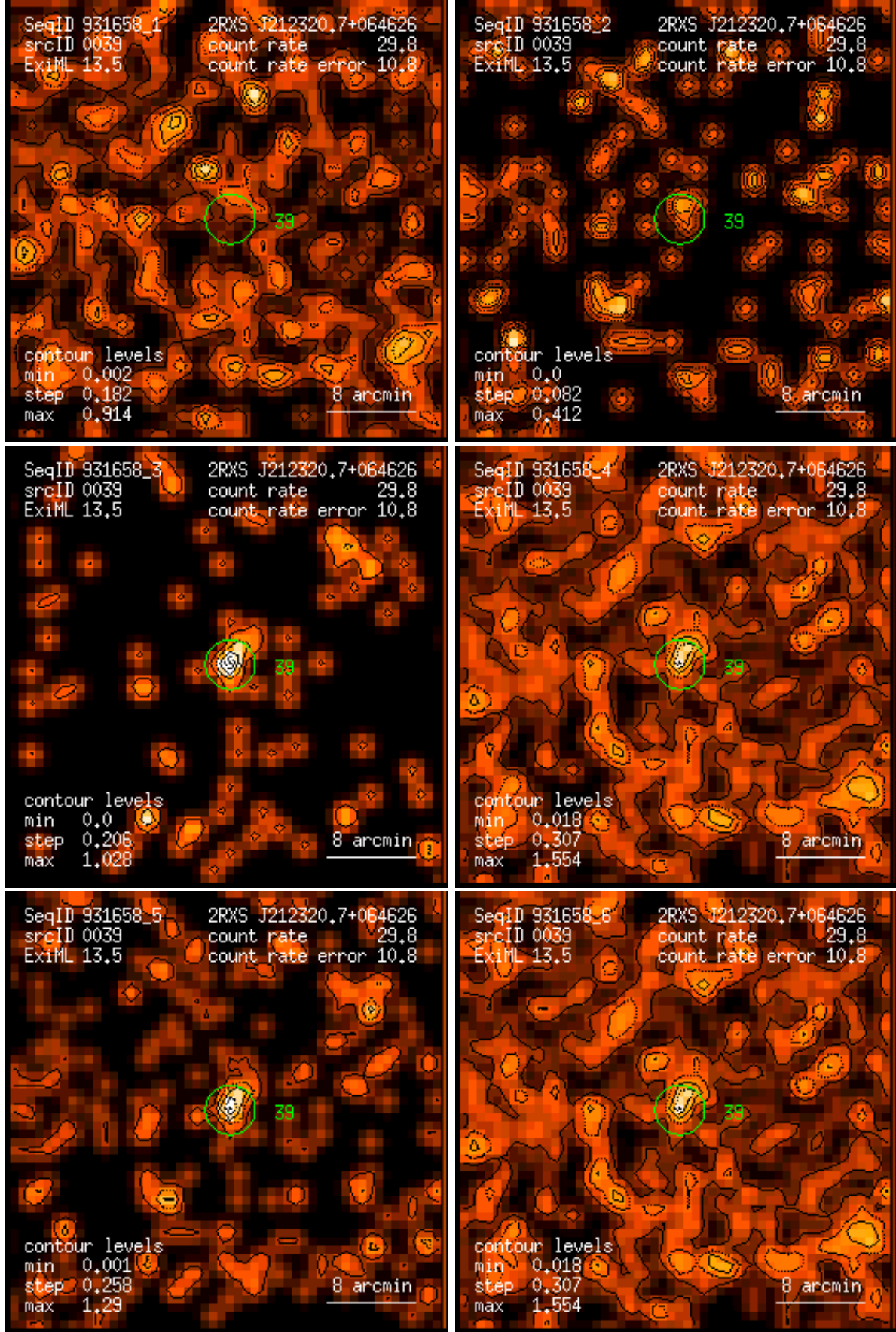
Figure 39: RASS 931658: detection 0039: band rate images, Gaussian filter: (1) PSPC channels 11 – 41, (2) 52 – 90, (3) 91 – 201, (4) 11 – 235, (5) 52 – 201, (6) 11 – 201. Broad band rates in counts/ks. Band rate contour levels in counts/ks/arcmin 2 .
