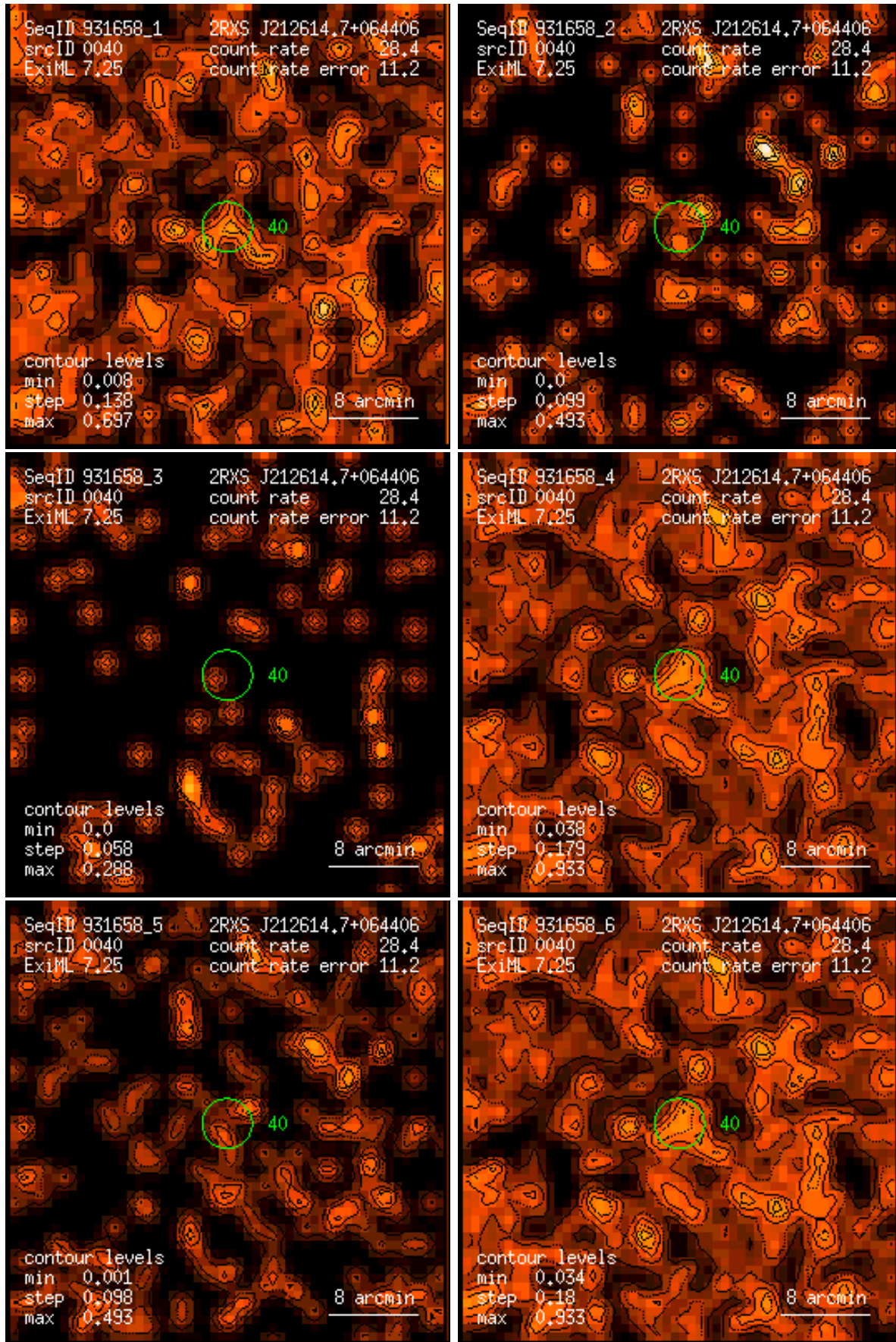
Figure 40: RASS 931658: detection 0040: band rate images, Gaussian filter: (1) PSPC channels 11 – 41, (2) 52 – 90, (3) 91 – 201, (4) 11 – 235, (5) 52 – 201, (6) 11 – 201. Broad band rates in counts/ks. Band rate contour levels in counts/ks/arcmin 2 .
