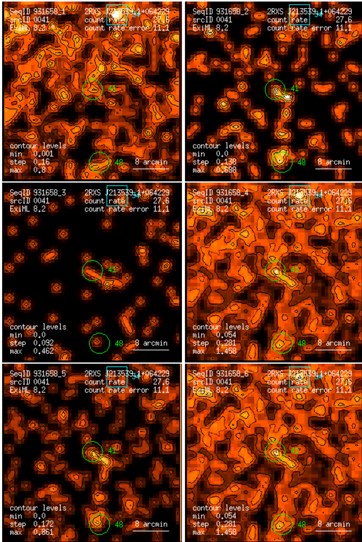
Figure 41: RASS 931658: detection 0041: band rate images, Gaussian filter: (1) PSPC channels 11 – 41, (2) 52 – 90, (3) 91 – 201, (4) 11 – 235, (5) 52 – 201, (6) 11 – 201. Broad band rates in counts/ks. Band rate contour levels in counts/ks/arcmin 2 .
