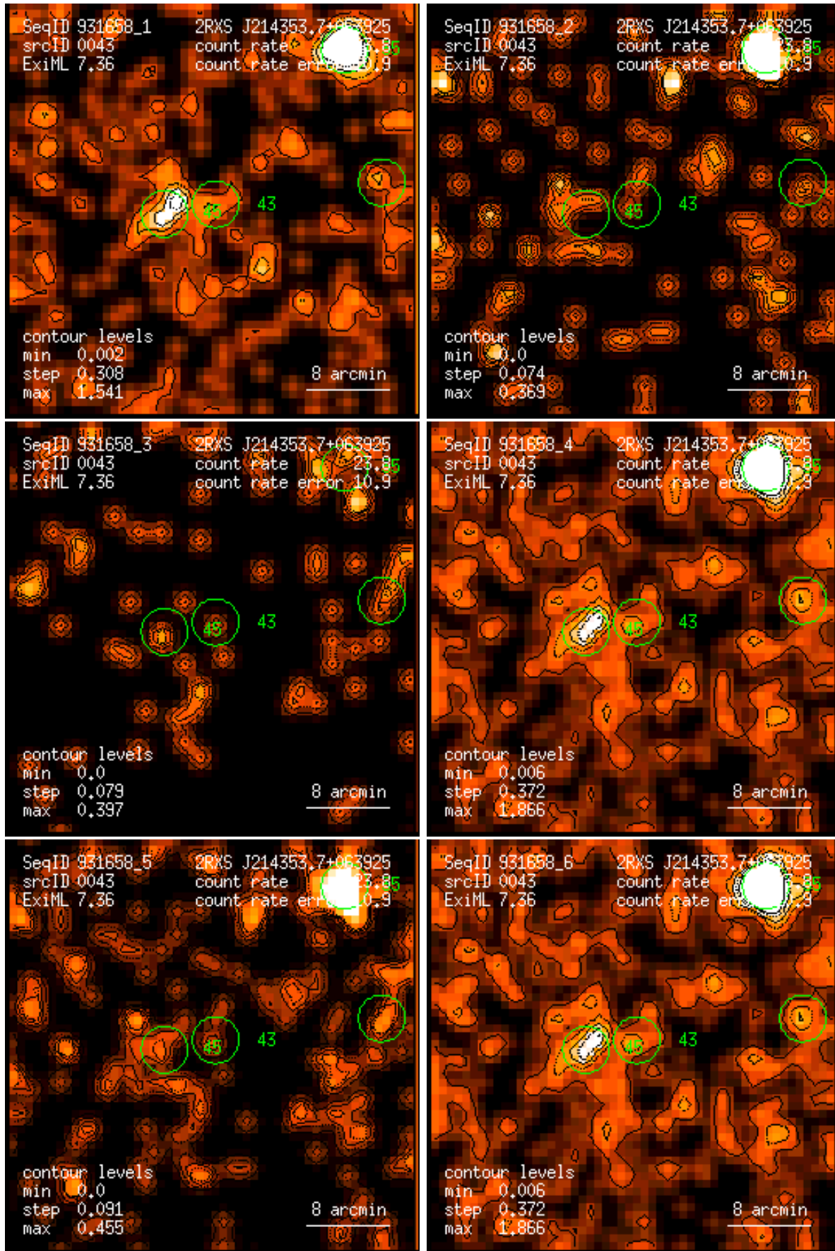
Figure 43: RASS 931658: detection 0043: band rate images, Gaussian filter: (1) PSPC channels 11 – 41, (2) 52 – 90, (3) 91 – 201, (4) 11 – 235, (5) 52 – 201, (6) 11 – 201. Broad band rates in counts/ks. Band rate contour levels in counts/ks/arcmin 2 .
