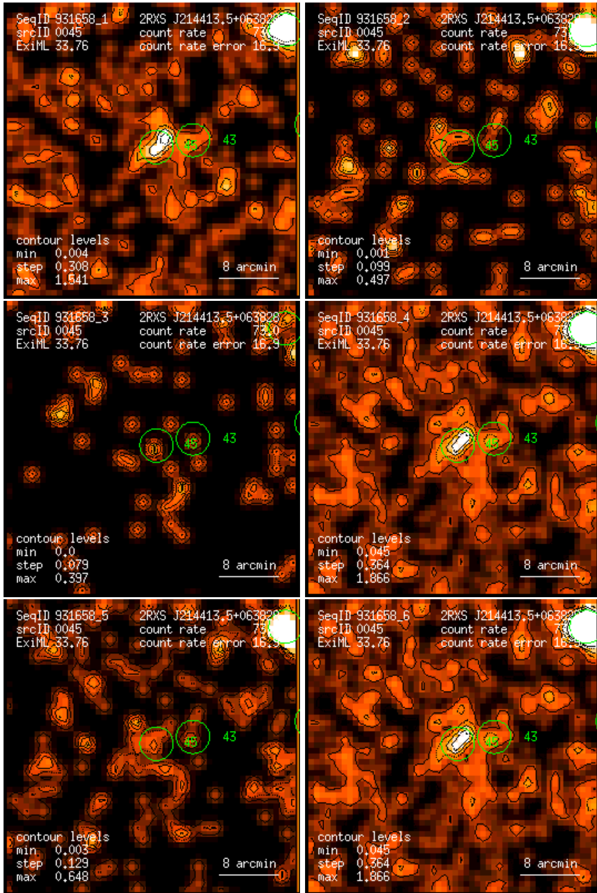
Figure 45: RASS 931658: detection 0045: band rate images, Gaussian filter: (1) PSPC channels 11 – 41, (2) 52 – 90, (3) 91 – 201, (4) 11 – 235, (5) 52 – 201, (6) 11 – 201. Broad band rates in counts/ks. Band rate contour levels in counts/ks/arcmin 2 .
