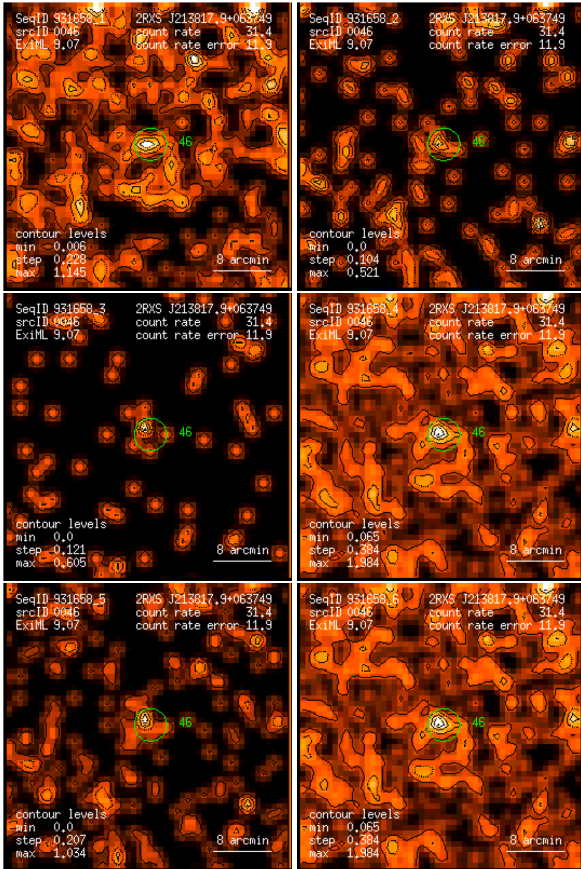
Figure 46: RASS 931658: detection 0046: band rate images, Gaussian filter: (1) PSPC channels 11 – 41, (2) 52 – 90, (3) 91 – 201, (4) 11 – 235, (5) 52 – 201, (6) 11 – 201. Broad band rates in counts/ks. Band rate contour levels in counts/ks/arcmin 2 .
