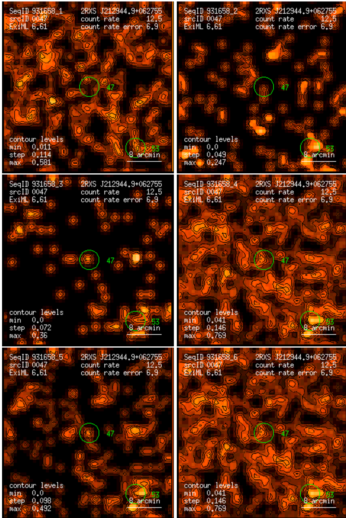
Figure 47: RASS 931658: detection 0047: band rate images, Gaussian filter: (1) PSPC channels 11 – 41, (2) 52 – 90, (3) 91 – 201, (4) 11 – 235, (5) 52 – 201, (6) 11 – 201. Broad band rates in counts/ks. Band rate contour levels in counts/ks/arcmin 2 .
