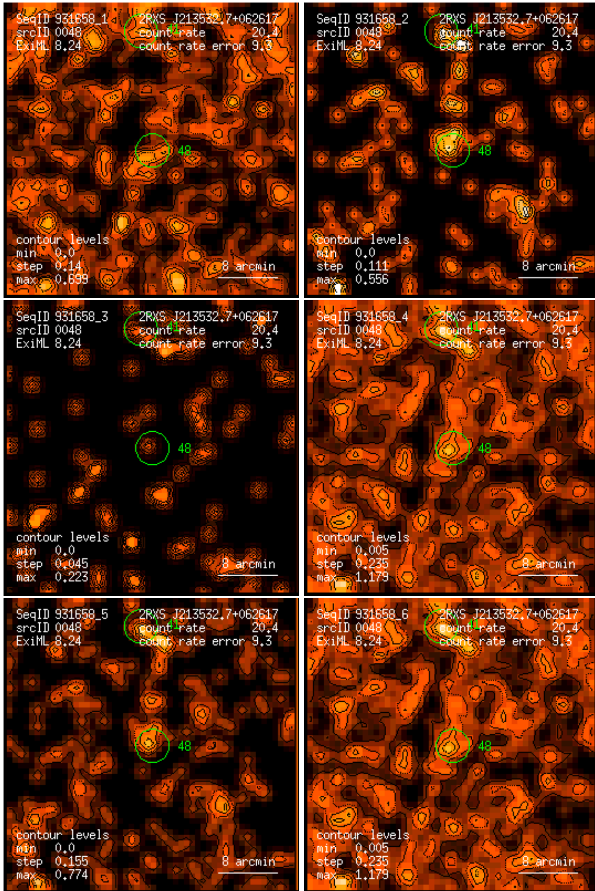
Figure 48: RASS 931658: detection 0048: band rate images, Gaussian filter: (1) PSPC channels 11 – 41, (2) 52 – 90, (3) 91 – 201, (4) 11 – 235, (5) 52 – 201, (6) 11 – 201. Broad band rates in counts/ks. Band rate contour levels in counts/ks/arcmin 2 .
