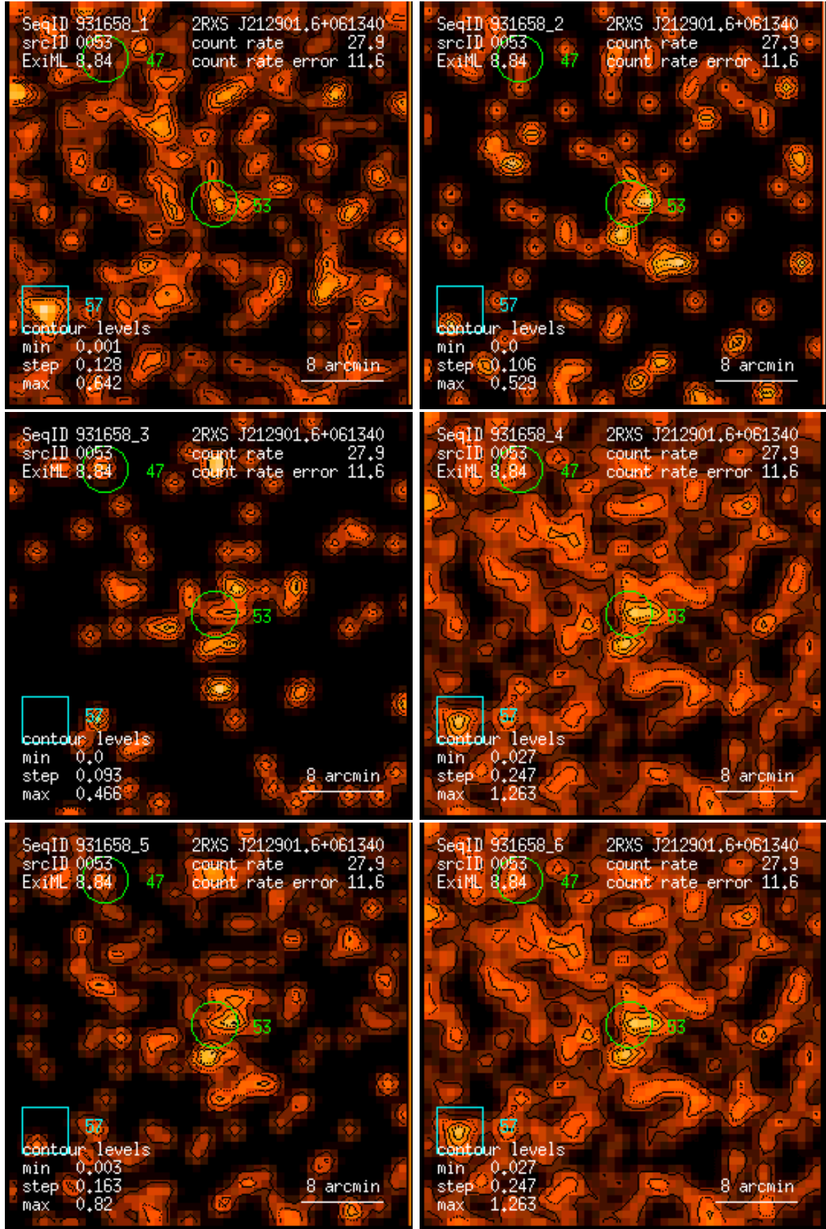
Figure 53: RASS 931658: detection 0053: band rate images, Gaussian filter: (1) PSPC channels 11 – 41, (2) 52 – 90, (3) 91 – 201, (4) 11 – 235, (5) 52 – 201, (6) 11 – 201. Broad band rates in counts/ks. Band rate contour levels in counts/ks/arcmin 2 .
