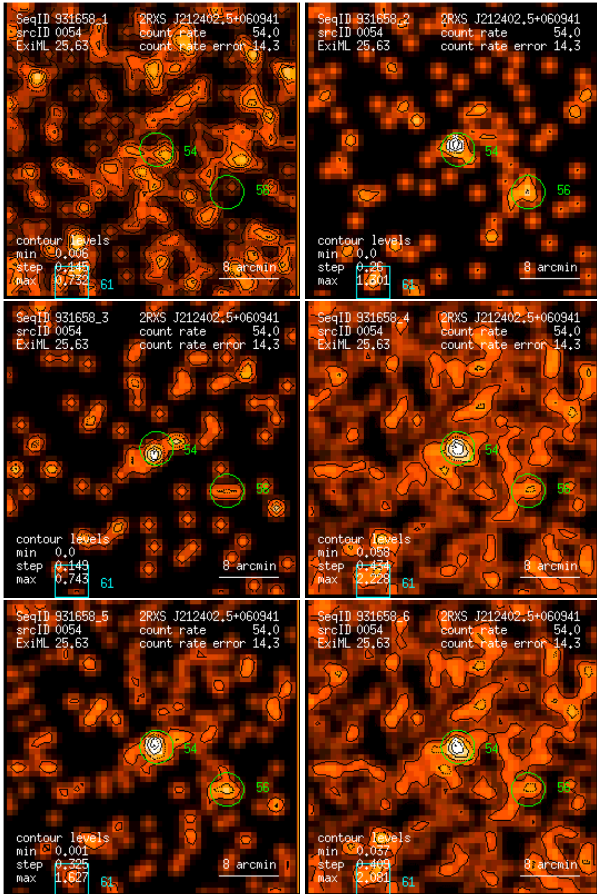
Figure 54: RASS 931658: detection 0054: band rate images, Gaussian filter: (1) PSPC channels 11 – 41, (2) 52 – 90, (3) 91 – 201, (4) 11 – 235, (5) 52 – 201, (6) 11 – 201. Broad band rates in counts/ks. Band rate contour levels in counts/ks/arcmin 2 .
