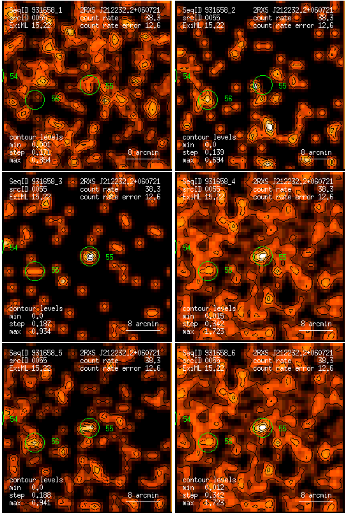
Figure 55: RASS 931658: detection 0055: band rate images, Gaussian filter: (1) PSPC channels 11 – 41, (2) 52 – 90, (3) 91 – 201, (4) 11 – 235, (5) 52 – 201, (6) 11 – 201. Broad band rates in counts/ks. Band rate contour levels in counts/ks/arcmin 2 .
