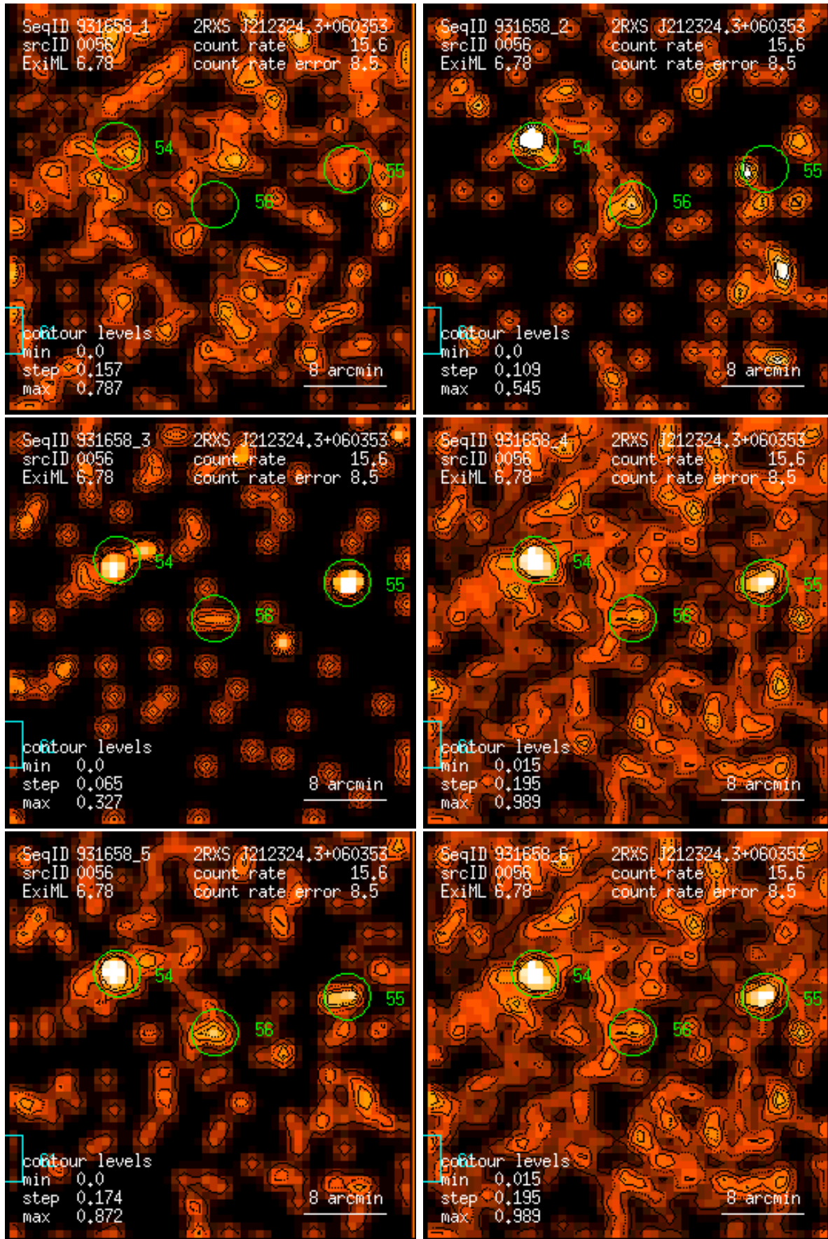
Figure 56: RASS 931658: detection 0056: band rate images, Gaussian filter: (1) PSPC channels 11 – 41, (2) 52 – 90, (3) 91 – 201, (4) 11 – 235, (5) 52 – 201, (6) 11 – 201. Broad band rates in counts/ks. Band rate contour levels in counts/ks/arcmin 2 .
