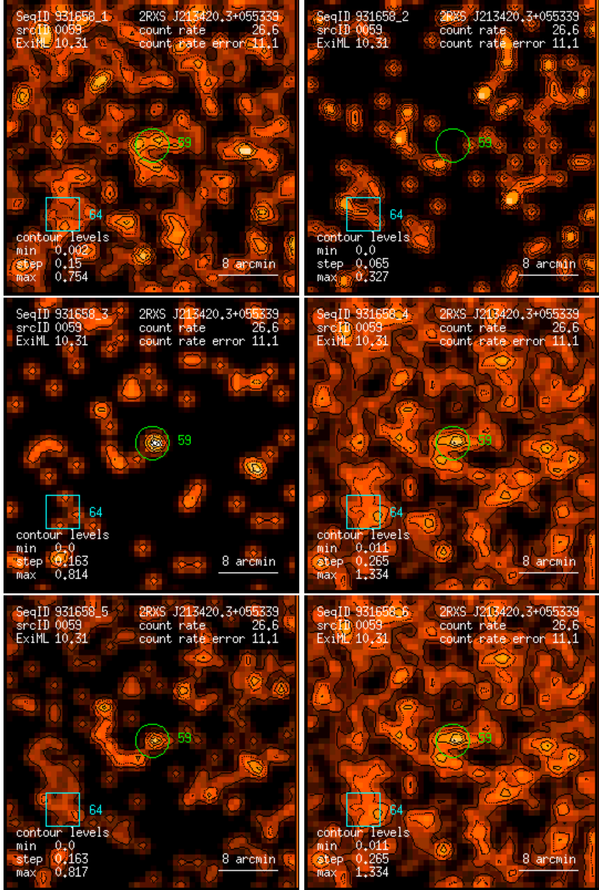
Figure 59: RASS 931658: detection 0059: band rate images, Gaussian filter: (1) PSPC channels 11 – 41, (2) 52 – 90, (3) 91 – 201, (4) 11 – 235, (5) 52 – 201, (6) 11 – 201. Broad band rates in counts/ks. Band rate contour levels in counts/ks/arcmin 2 .
