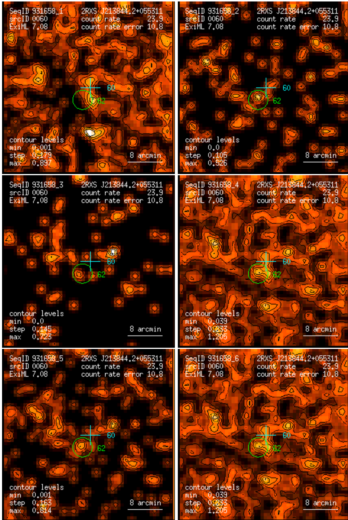
Figure 60: RASS 931658: detection 0060: band rate images, Gaussian filter: (1) PSPC channels 11 – 41, (2) 52 – 90, (3) 91 – 201, (4) 11 – 235, (5) 52 – 201, (6) 11 – 201. Broad band rates in counts/ks. Band rate contour levels in counts/ks/arcmin 2 .
