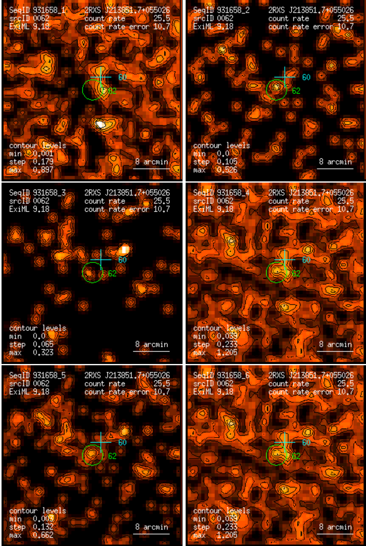
Figure 62: RASS 931658: detection 0062: band rate images, Gaussian filter: (1) PSPC channels 11 – 41, (2) 52 – 90, (3) 91 – 201, (4) 11 – 235, (5) 52 – 201, (6) 11 – 201. Broad band rates in counts/ks. Band rate contour levels in counts/ks/arcmin 2 .
