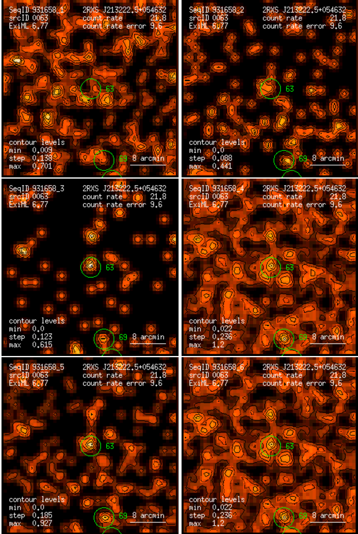
Figure 63: RASS 931658: detection 0063: band rate images, Gaussian filter: (1) PSPC channels 11 – 41, (2) 52 – 90, (3) 91 – 201, (4) 11 – 235, (5) 52 – 201, (6) 11 – 201. Broad band rates in counts/ks. Band rate contour levels in counts/ks/arcmin 2 .
