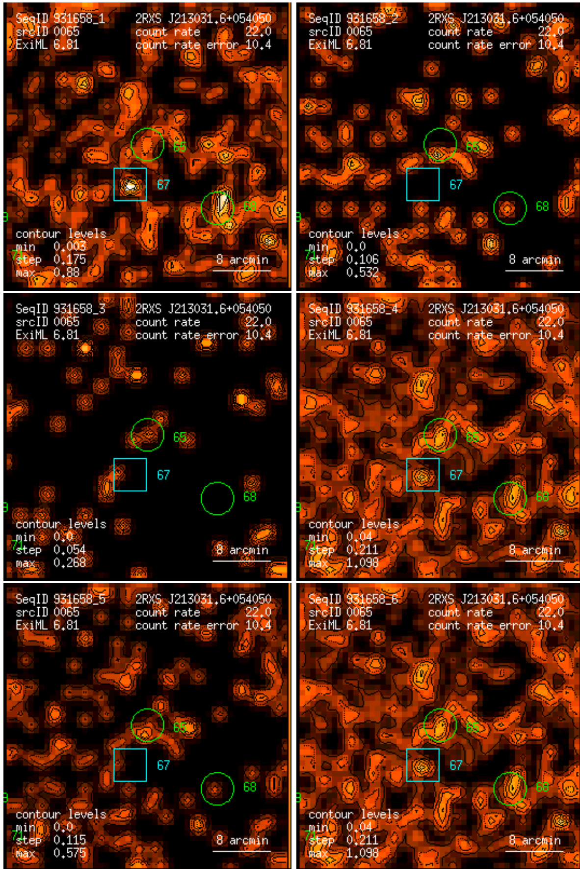
Figure 65: RASS 931658: detection 0065: band rate images, Gaussian filter: (1) PSPC channels 11 – 41, (2) 52 – 90, (3) 91 – 201, (4) 11 – 235, (5) 52 – 201, (6) 11 – 201. Broad band rates in counts/ks. Band rate contour levels in counts/ks/arcmin 2 .
