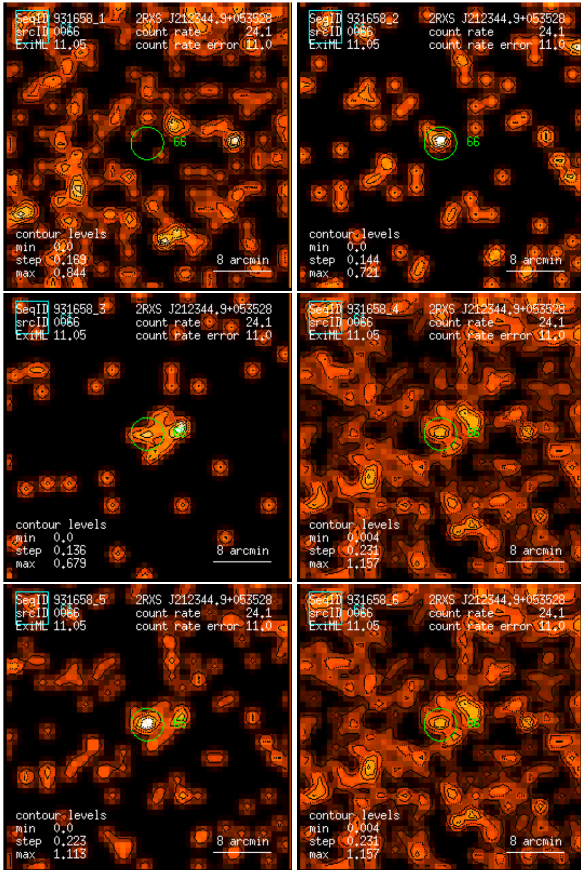
Figure 66: RASS 931658: detection 0066: band rate images, Gaussian filter: (1) PSPC channels 11 – 41, (2) 52 – 90, (3) 91 – 201, (4) 11 – 235, (5) 52 – 201, (6) 11 – 201. Broad band rates in counts/ks. Band rate contour levels in counts/ks/arcmin 2 .
