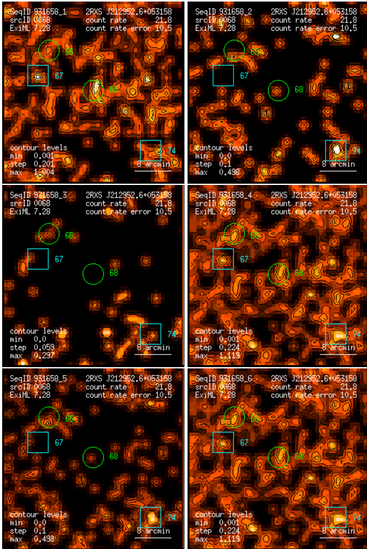
Figure 68: RASS 931658: detection 0068: band rate images, Gaussian filter: (1) PSPC channels 11 – 41, (2) 52 – 90, (3) 91 – 201, (4) 11 – 235, (5) 52 – 201, (6) 11 – 201. Broad band rates in counts/ks. Band rate contour levels in counts/ks/arcmin 2 .
