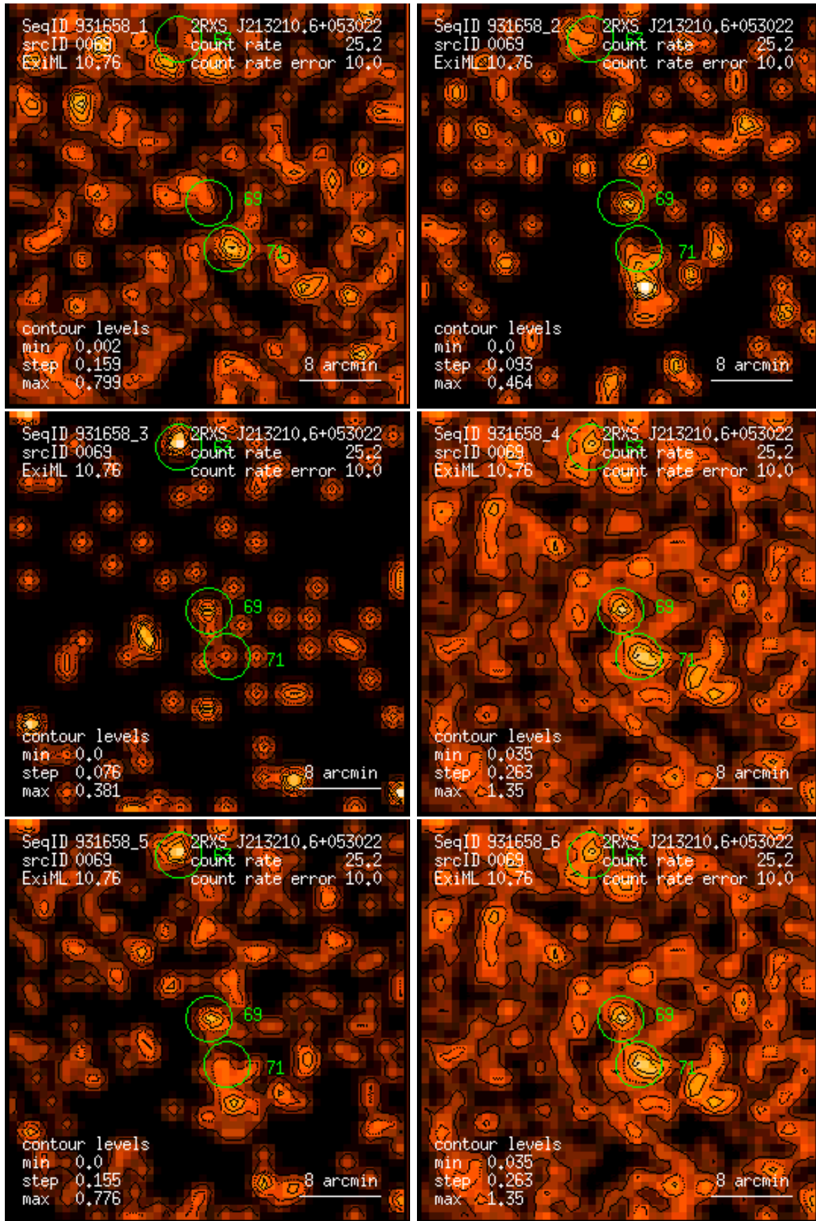
Figure 69: RASS 931658: detection 0069: band rate images, Gaussian filter: (1) PSPC channels 11 – 41, (2) 52 – 90, (3) 91 – 201, (4) 11 – 235, (5) 52 – 201, (6) 11 – 201. Broad band rates in counts/ks. Band rate contour levels in counts/ks/arcmin 2 .
