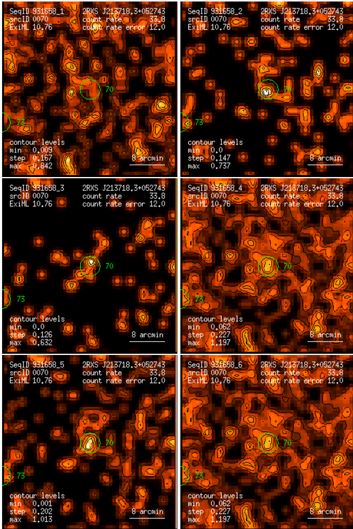
Figure 70: RASS 931658: detection 0070: band rate images, Gaussian filter: (1) PSPC channels 11 – 41, (2) 52 – 90, (3) 91 – 201, (4) 11 – 235, (5) 52 – 201, (6) 11 – 201. Broad band rates in counts/ks. Band rate contour levels in counts/ks/arcmin 2 .
