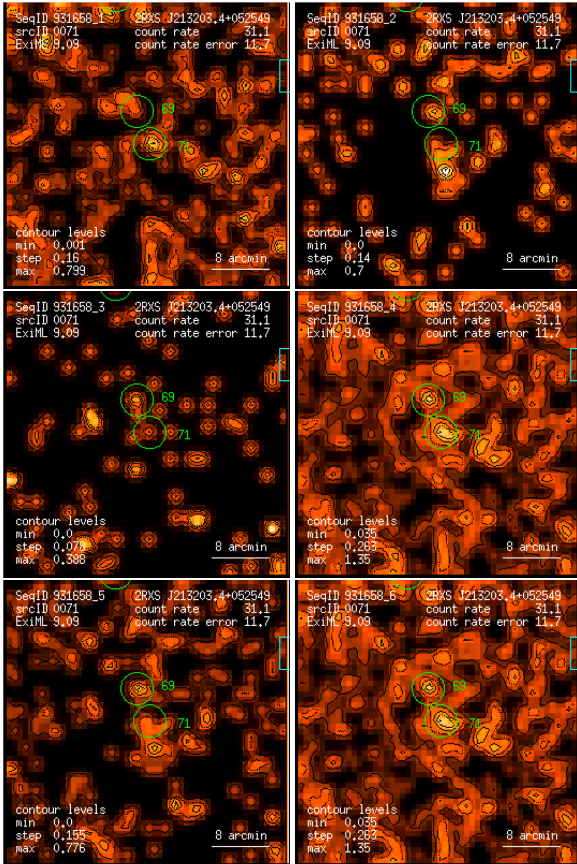
Figure 71: RASS 931658: detection 0071: band rate images, Gaussian filter: (1) PSPC channels 11 – 41, (2) 52 – 90, (3) 91 – 201, (4) 11 – 235, (5) 52 – 201, (6) 11 – 201. Broad band rates in counts/ks. Band rate contour levels in counts/ks/arcmin 2 .
