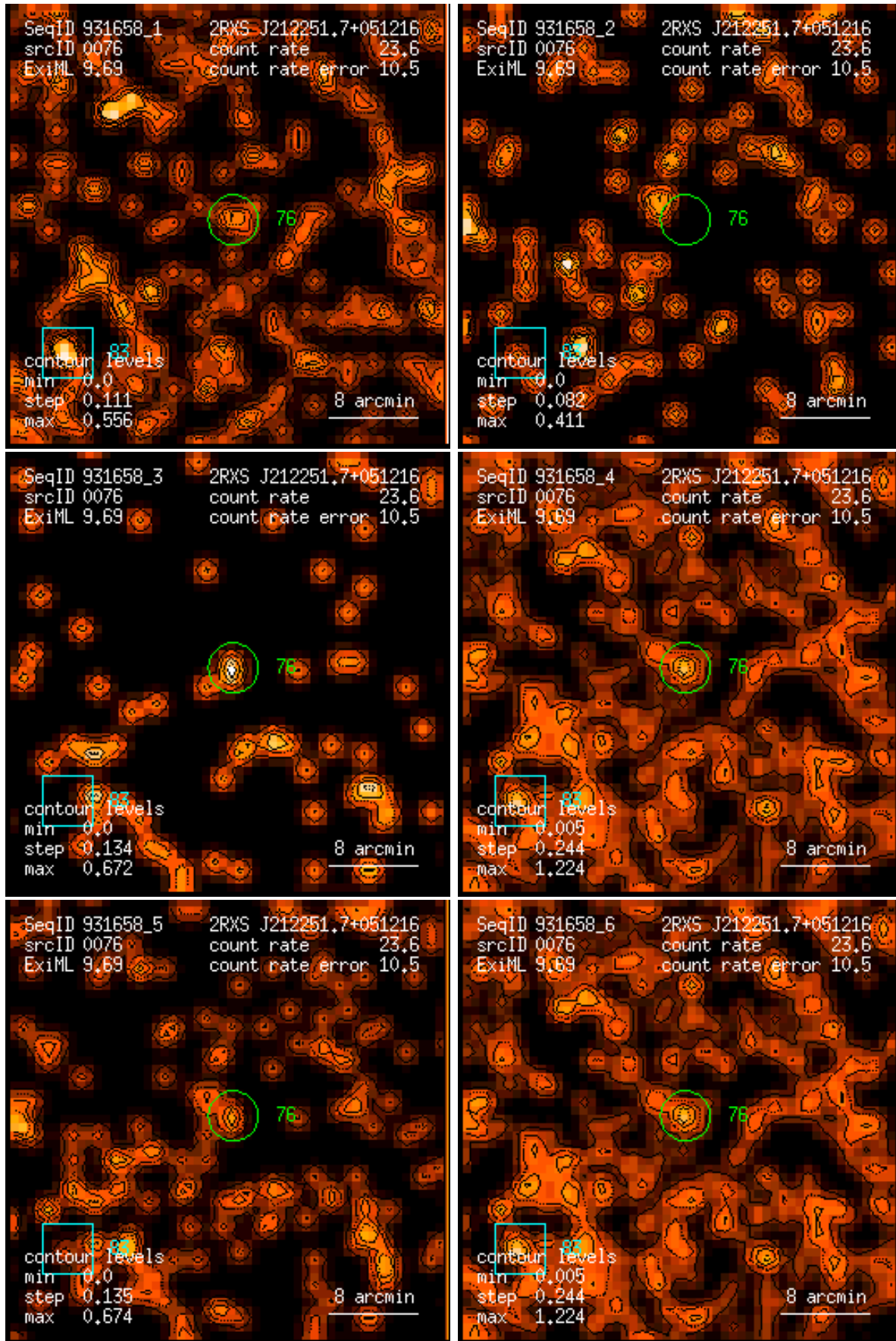
Figure 76: RASS 931658: detection 0076: band rate images, Gaussian filter: (1) PSPC channels 11 – 41, (2) 52 – 90, (3) 91 – 201, (4) 11 – 235, (5) 52 – 201, (6) 11 – 201. Broad band rates in counts/ks. Band rate contour levels in counts/ks/arcmin 2 .
