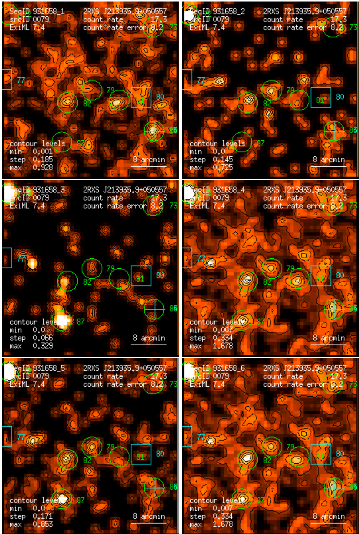
Figure 79: RASS 931658: detection 0079: band rate images, Gaussian filter: (1) PSPC channels 11 – 41, (2) 52 – 90, (3) 91 – 201, (4) 11 – 235, (5) 52 – 201, (6) 11 – 201. Broad band rates in counts/ks. Band rate contour levels in counts/ks/arcmin 2 .
