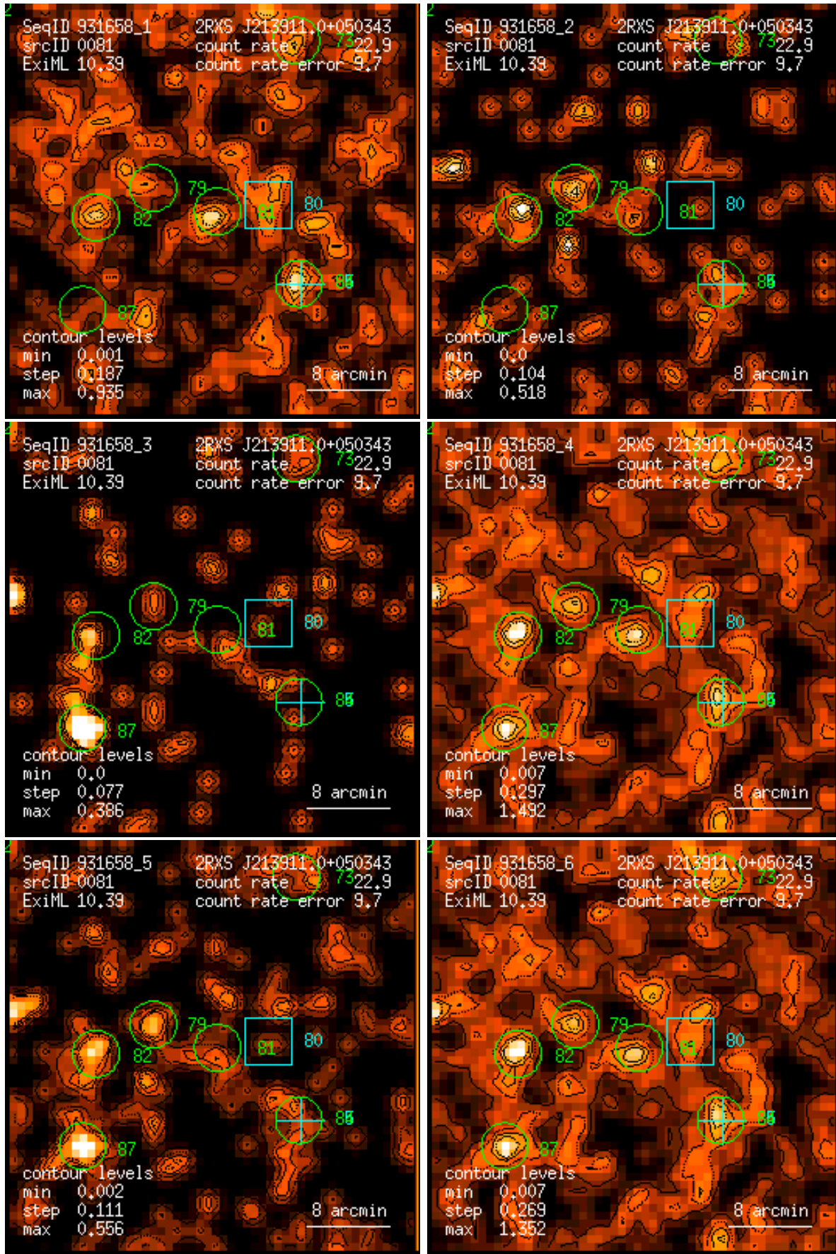
Figure 81: RASS 931658: detection 0081: band rate images, Gaussian filter: (1) PSPC channels 11 – 41, (2) 52 – 90, (3) 91 – 201, (4) 11 – 235, (5) 52 – 201, (6) 11 – 201. Broad band rates in counts/ks. Band rate contour levels in counts/ks/arcmin 2 .
