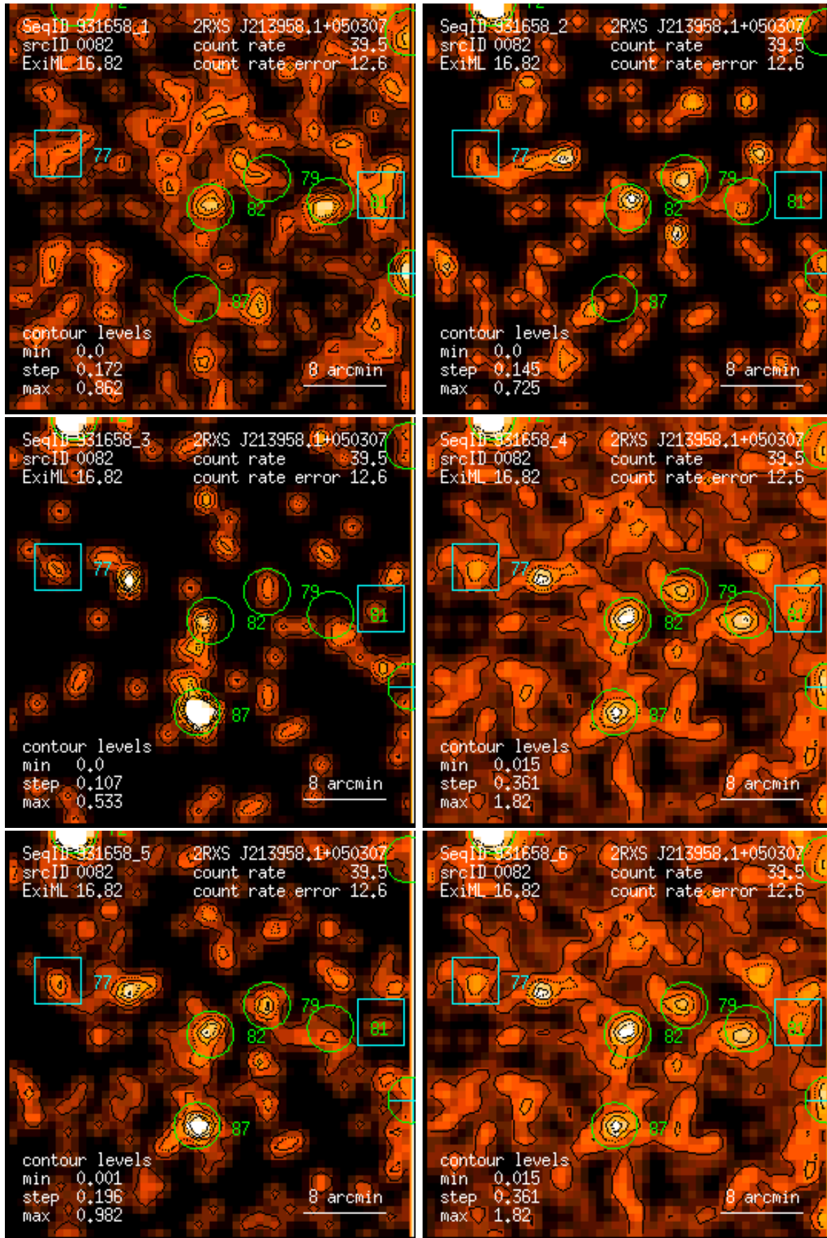
Figure 82: RASS 931658: detection 0082: band rate images, Gaussian filter: (1) PSPC channels 11 – 41, (2) 52 – 90, (3) 91 – 201, (4) 11 – 235, (5) 52 – 201, (6) 11 – 201. Broad band rates in counts/ks. Band rate contour levels in counts/ks/arcmin 2 .
