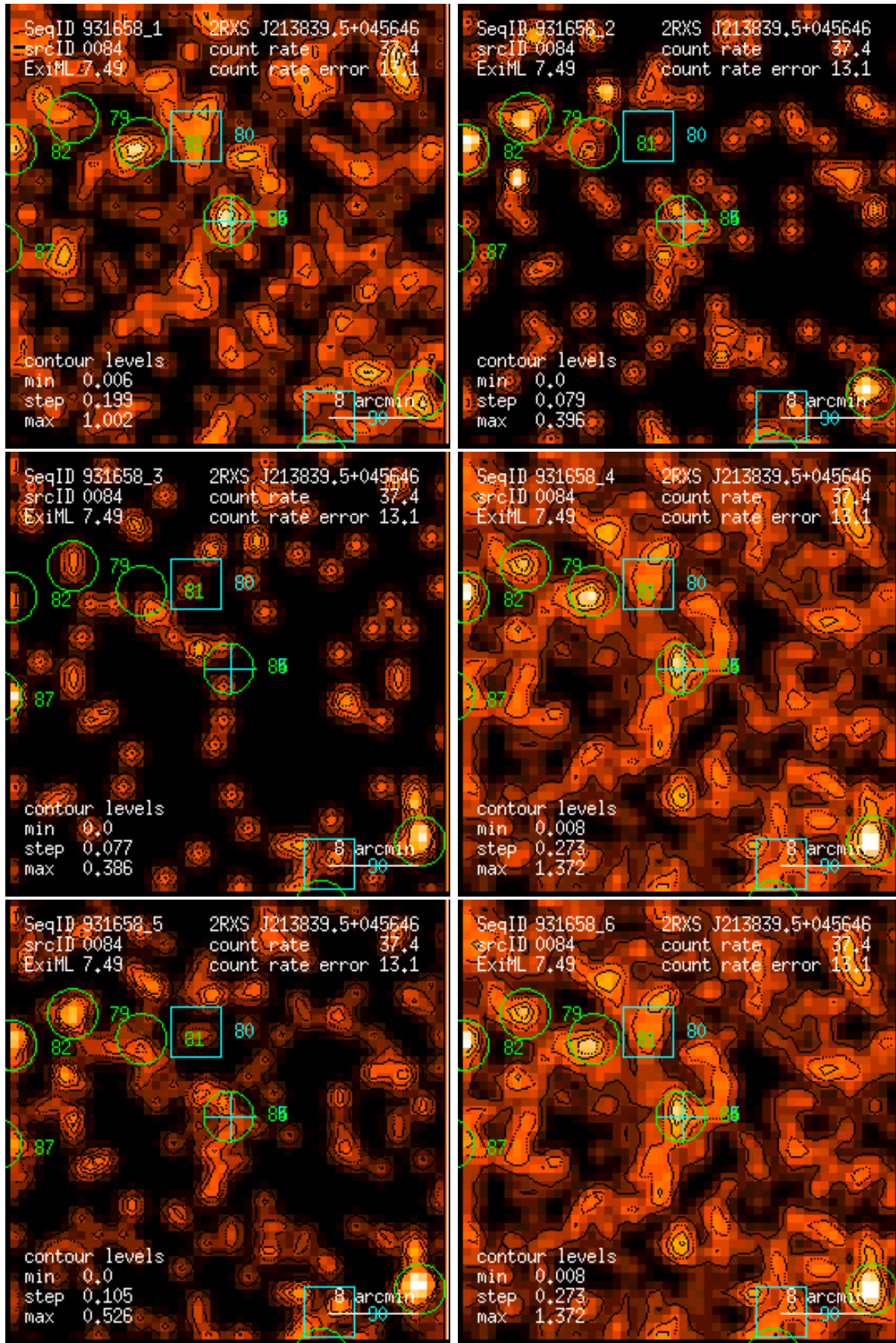
Figure 84: RASS 931658: detection 0084: band rate images, Gaussian filter: (1) PSPC channels 11 – 41, (2) 52 – 90, (3) 91 – 201, (4) 11 – 235, (5) 52 – 201, (6) 11 – 201. Broad band rates in counts/ks. Band rate contour levels in counts/ks/arcmin 2 .
