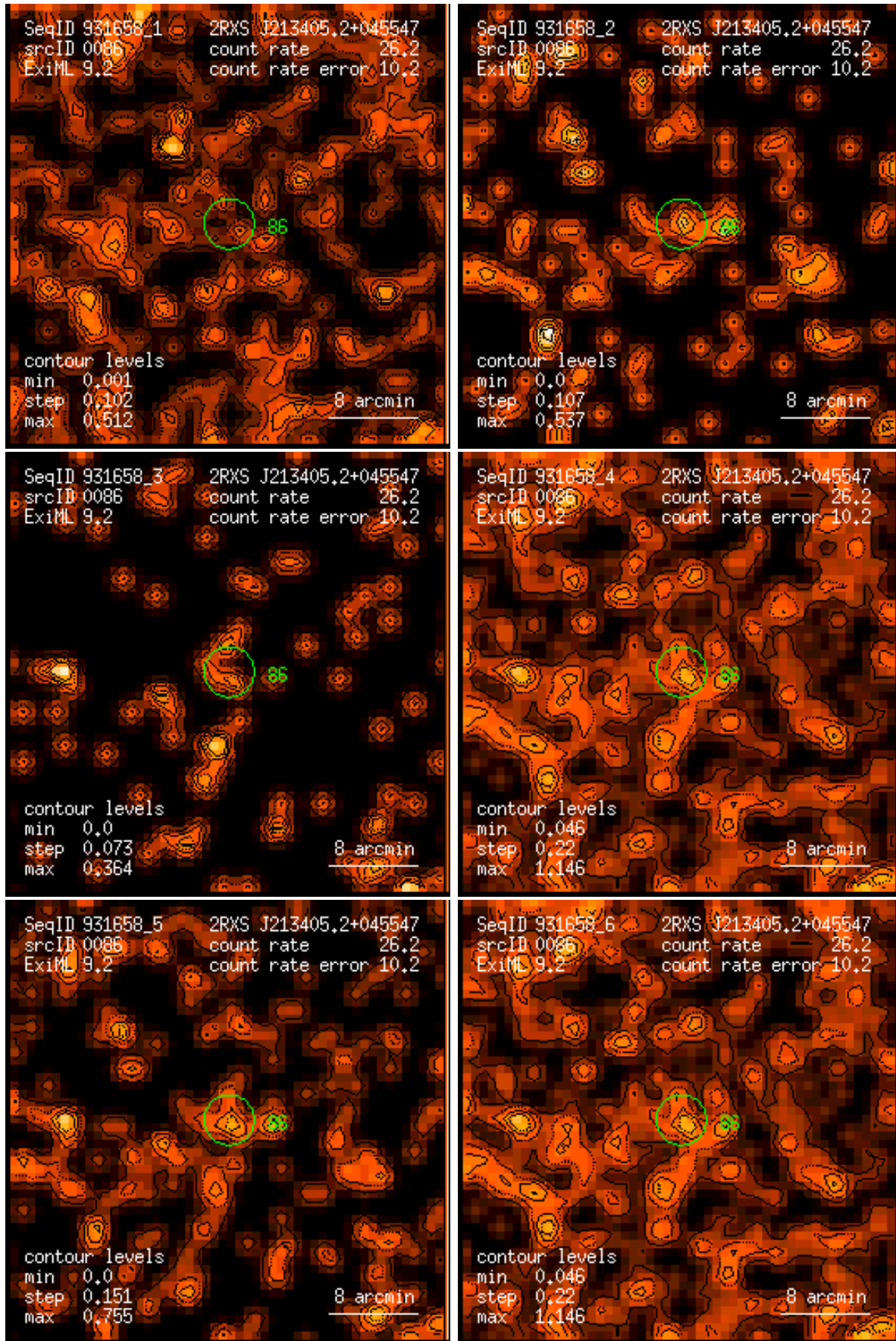
Figure 86: RASS 931658: detection 0086: band rate images, Gaussian filter: (1) PSPC channels 11 – 41, (2) 52 – 90, (3) 91 – 201, (4) 11 – 235, (5) 52 – 201, (6) 11 – 201. Broad band rates in counts/ks. Band rate contour levels in counts/ks/arcmin 2 .
