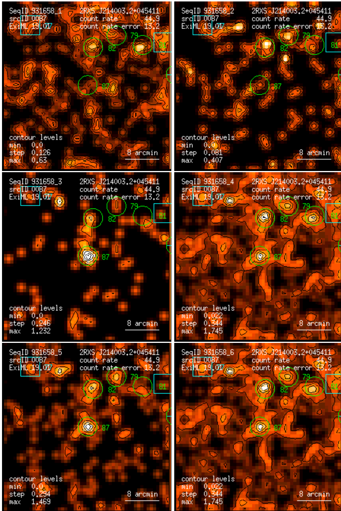
Figure 87: RASS 931658: detection 0087: band rate images, Gaussian filter: (1) PSPC channels 11 – 41, (2) 52 – 90, (3) 91 – 201, (4) 11 – 235, (5) 52 – 201, (6) 11 – 201. Broad band rates in counts/ks. Band rate contour levels in counts/ks/arcmin 2 .
