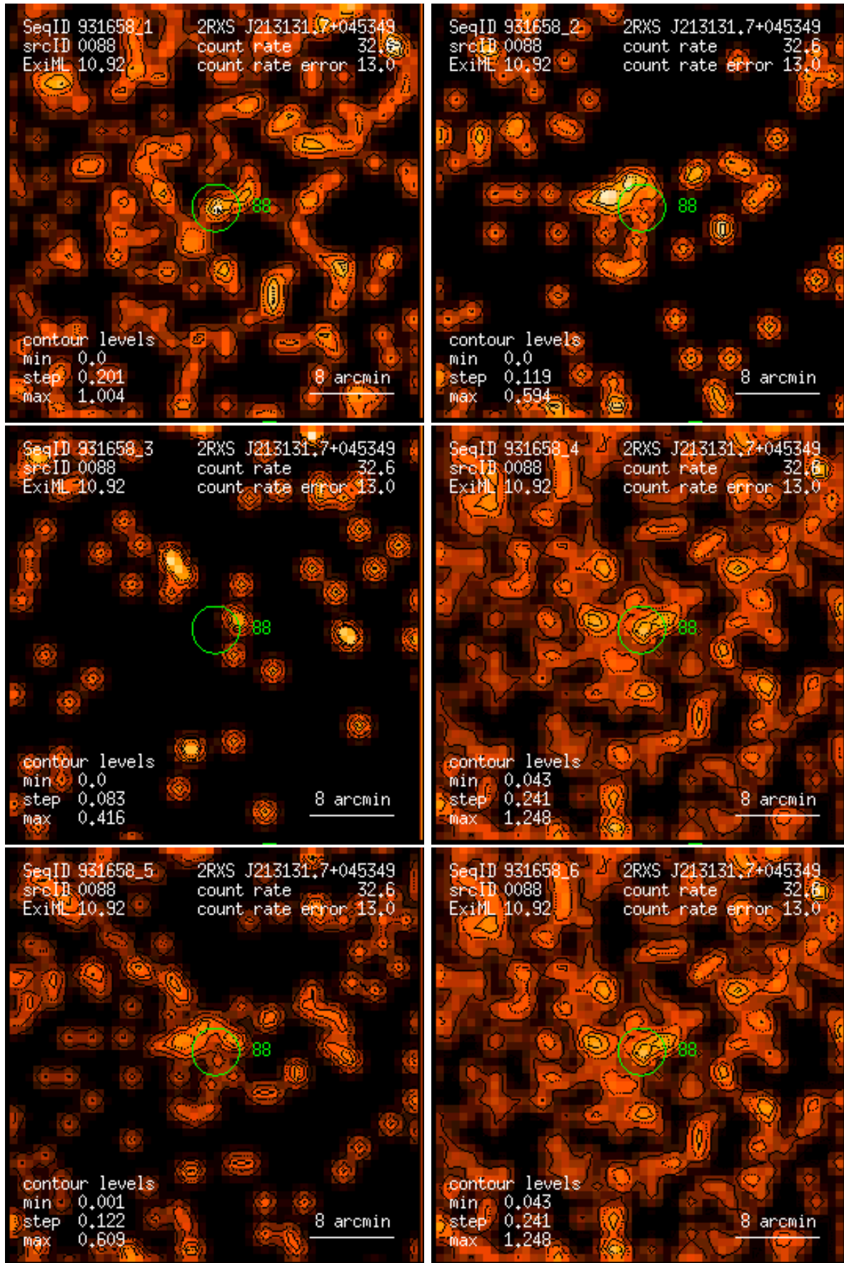
Figure 88: RASS 931658: detection 0088: band rate images, Gaussian filter: (1) PSPC channels 11 – 41, (2) 52 – 90, (3) 91 – 201, (4) 11 – 235, (5) 52 – 201, (6) 11 – 201. Broad band rates in counts/ks. Band rate contour levels in counts/ks/arcmin 2 .
