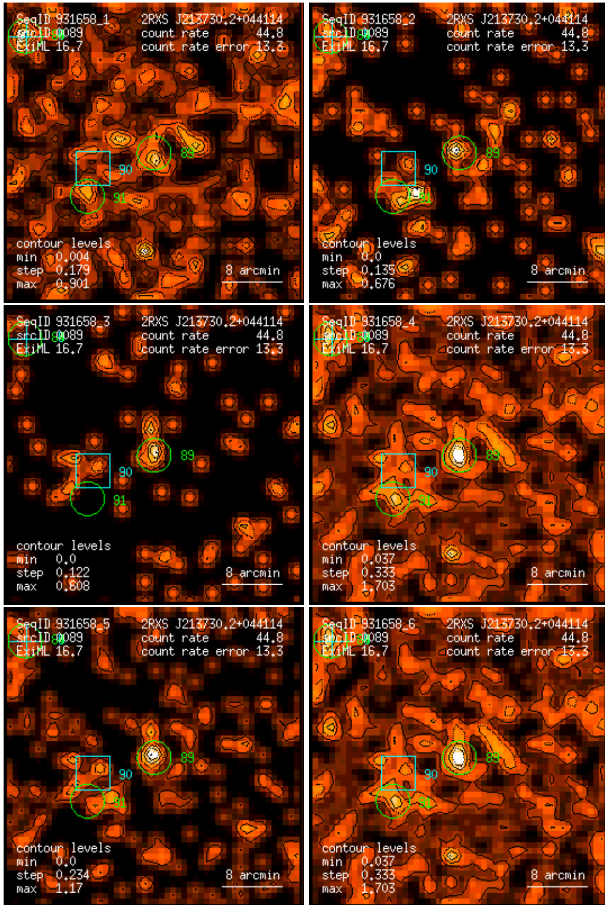
Figure 89: RASS 931658: detection 0089: band rate images, Gaussian filter: (1) PSPC channels 11 – 41, (2) 52 – 90, (3) 91 – 201, (4) 11 – 235, (5) 52 – 201, (6) 11 – 201. Broad band rates in counts/ks. Band rate contour levels in counts/ks/arcmin 2 .
