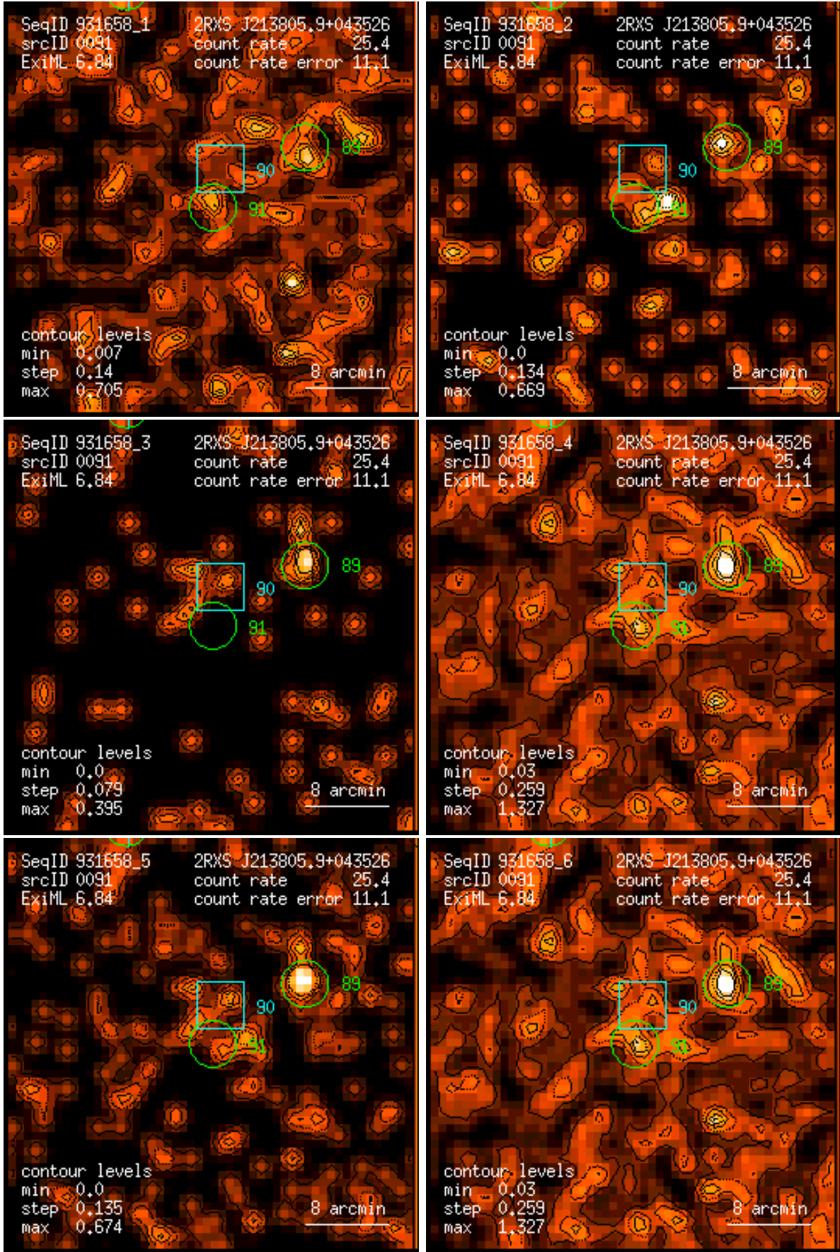
Figure 91: RASS 931658: detection 0091: band rate images, Gaussian filter: (1) PSPC channels 11 – 41, (2) 52 – 90, (3) 91 – 201, (4) 11 – 235, (5) 52 – 201, (6) 11 – 201. Broad band rates in counts/ks. Band rate contour levels in counts/ks/arcmin 2 .
