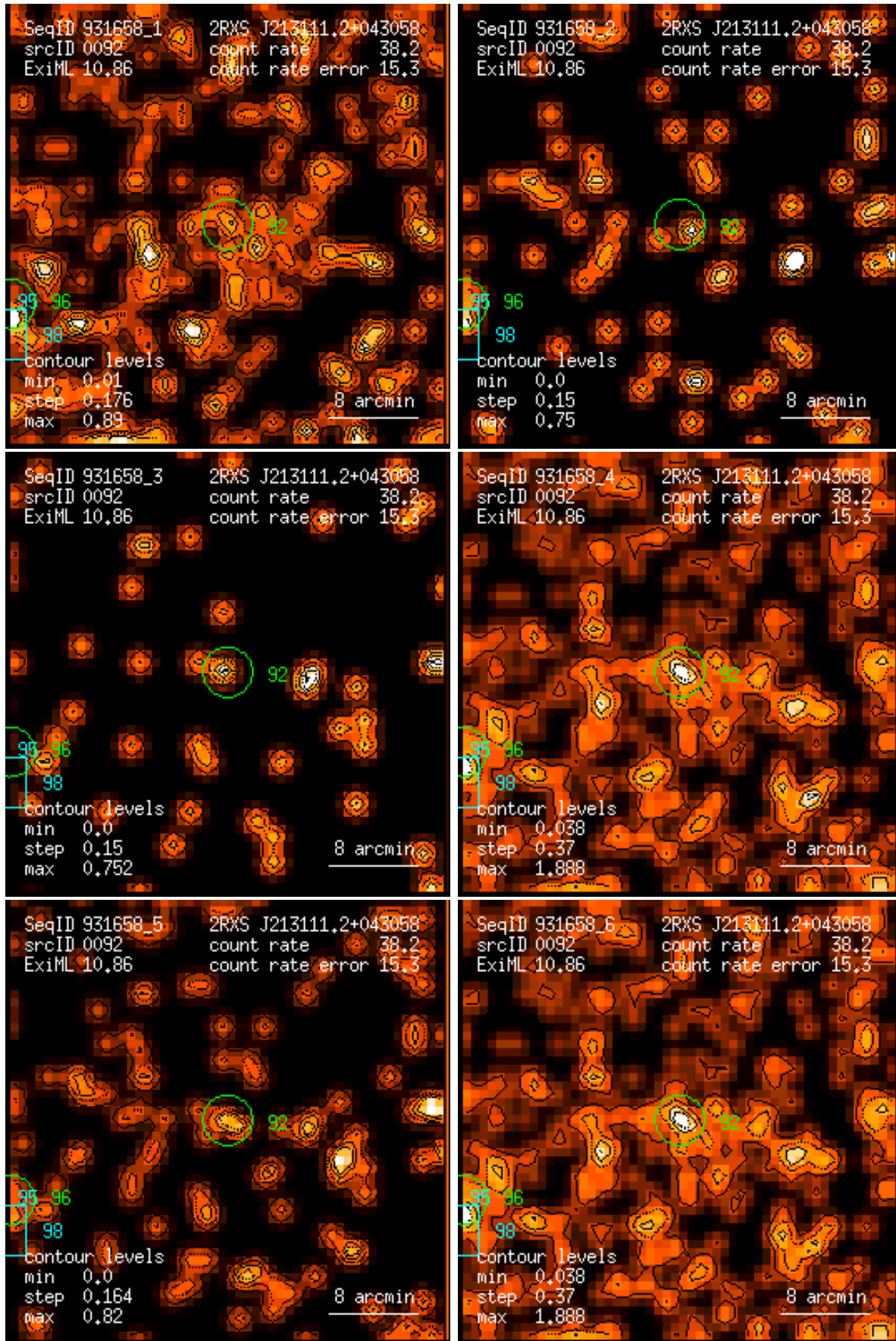
Figure 92: RASS 931658: detection 0092: band rate images, Gaussian filter: (1) PSPC channels 11 – 41, (2) 52 – 90, (3) 91 – 201, (4) 11 – 235, (5) 52 – 201, (6) 11 – 201. Broad band rates in counts/ks. Band rate contour levels in counts/ks/arcmin 2 .
