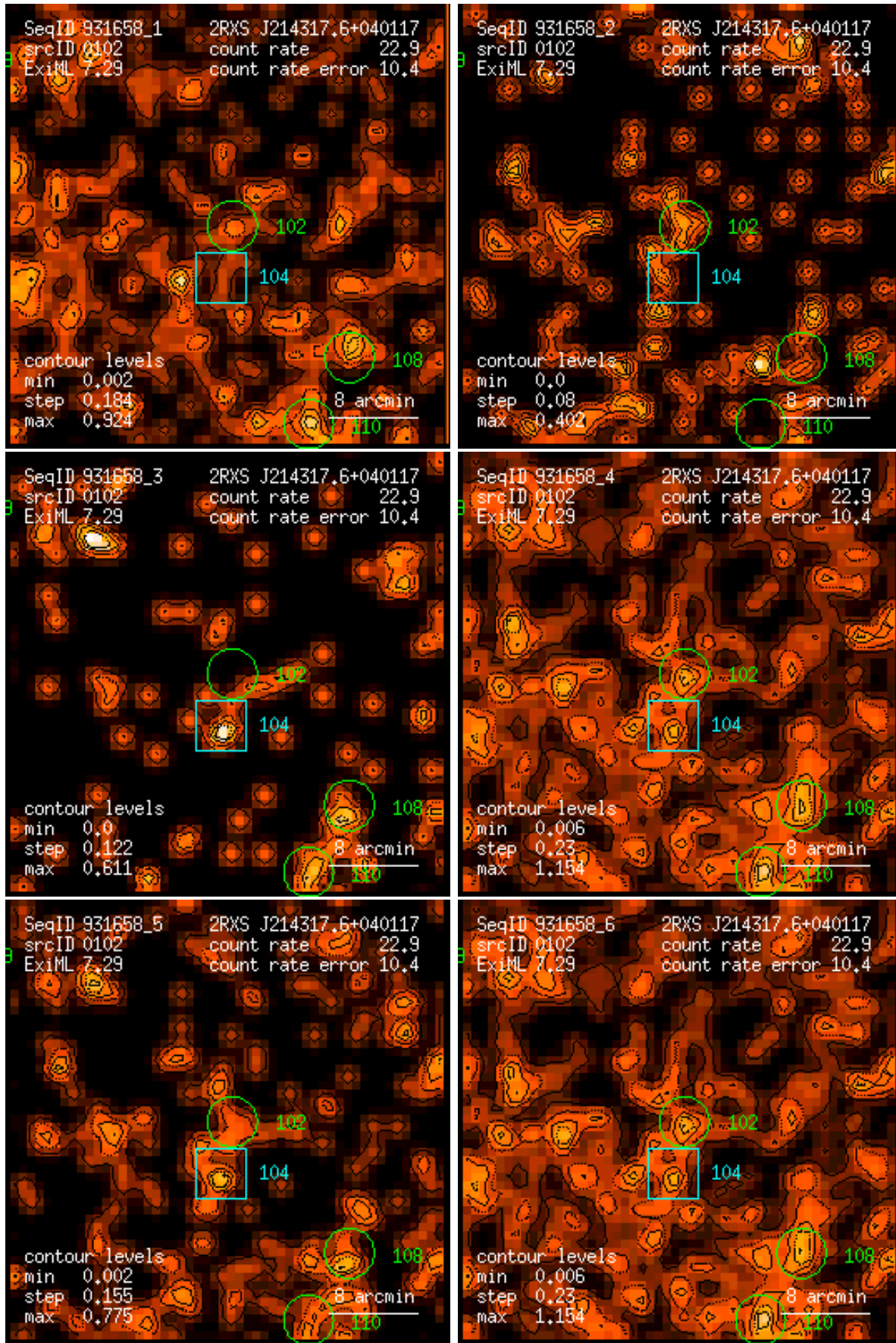
Figure 102: RASS 931658: detection 0102: band rate images, Gaussian filter: (1) PSPC channels 11 – 41, (2) 52 – 90, (3) 91 – 201, (4) 11 – 235, (5) 52 – 201, (6) 11 – 201. Broad band rates in counts/ks. Band rate contour levels in counts/ks/arcmin 2 .
