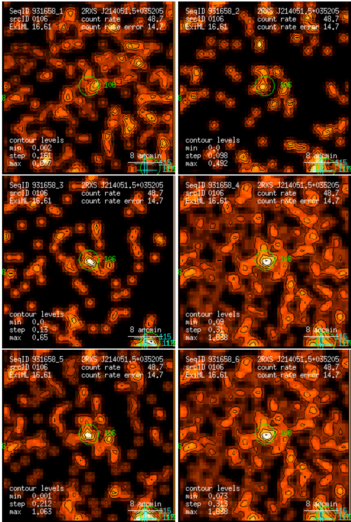
Figure 106: RASS 931658: detection 0106: band rate images, Gaussian filter: (1) PSPC channels 11 – 41, (2) 52 – 90, (3) 91 – 201, (4) 11 – 235, (5) 52 – 201, (6) 11 – 201. Broad band rates in counts/ks. Band rate contour levels in counts/ks/arcmin 2 .
