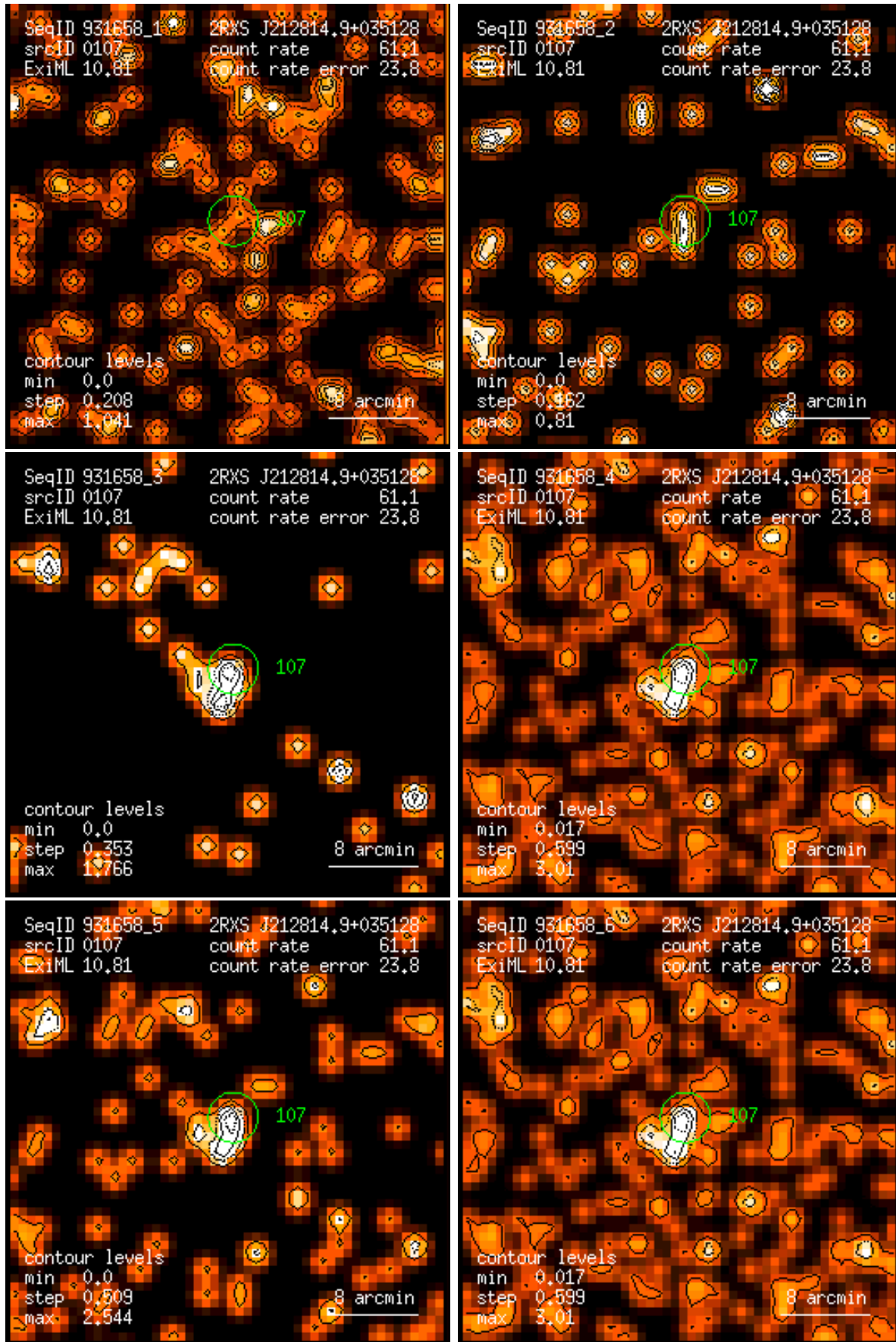
Figure 107: RASS 931658: detection 0107: band rate images, Gaussian filter: (1) PSPC channels 11 – 41, (2) 52 – 90, (3) 91 – 201, (4) 11 – 235, (5) 52 – 201, (6) 11 – 201. Broad band rates in counts/ks. Band rate contour levels in counts/ks/arcmin 2 .
