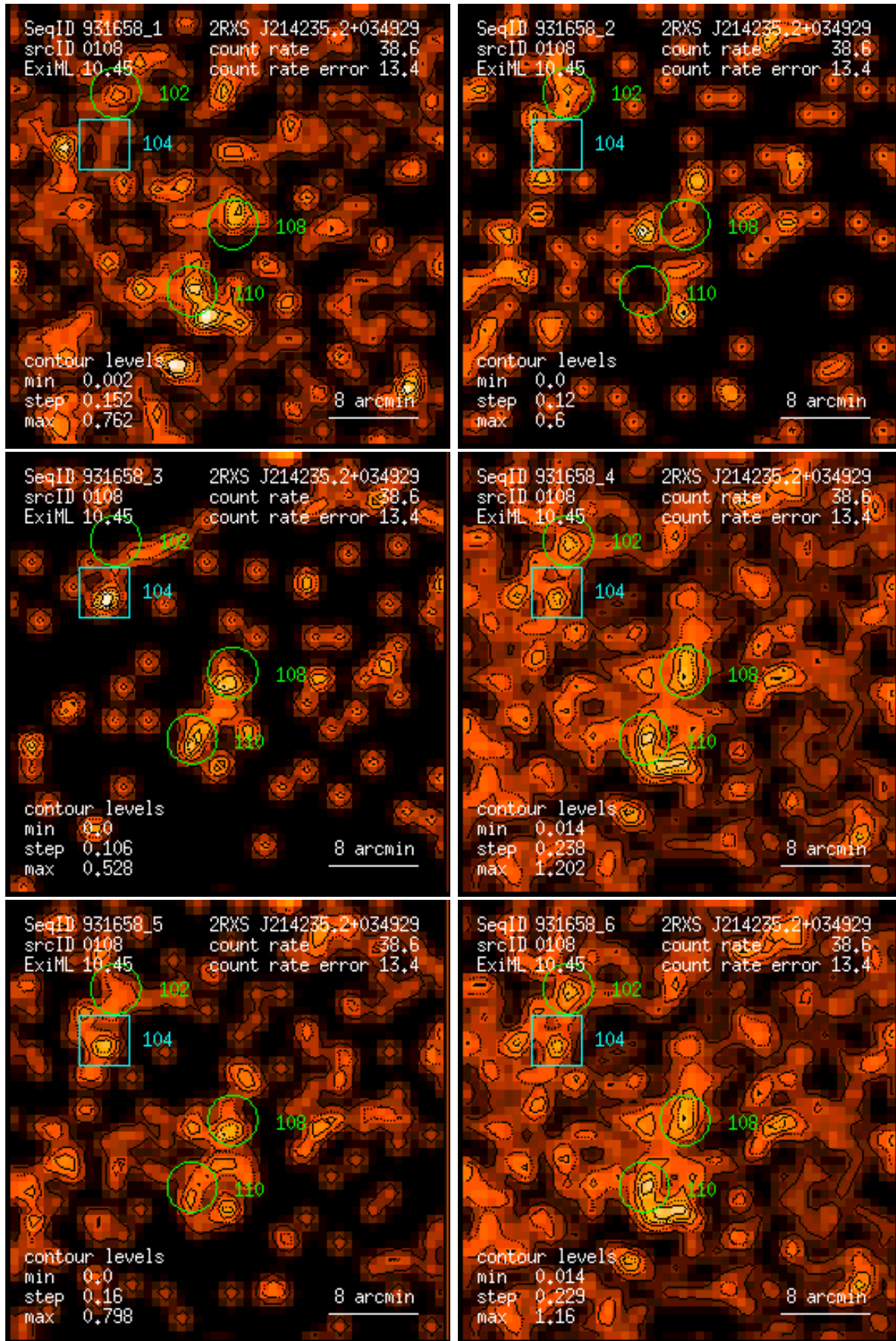
Figure 108: RASS 931658: detection 0108: band rate images, Gaussian filter: (1) PSPC channels 11 – 41, (2) 52 – 90, (3) 91 – 201, (4) 11 – 235, (5) 52 – 201, (6) 11 – 201. Broad band rates in counts/ks. Band rate contour levels in counts/ks/arcmin 2 .
