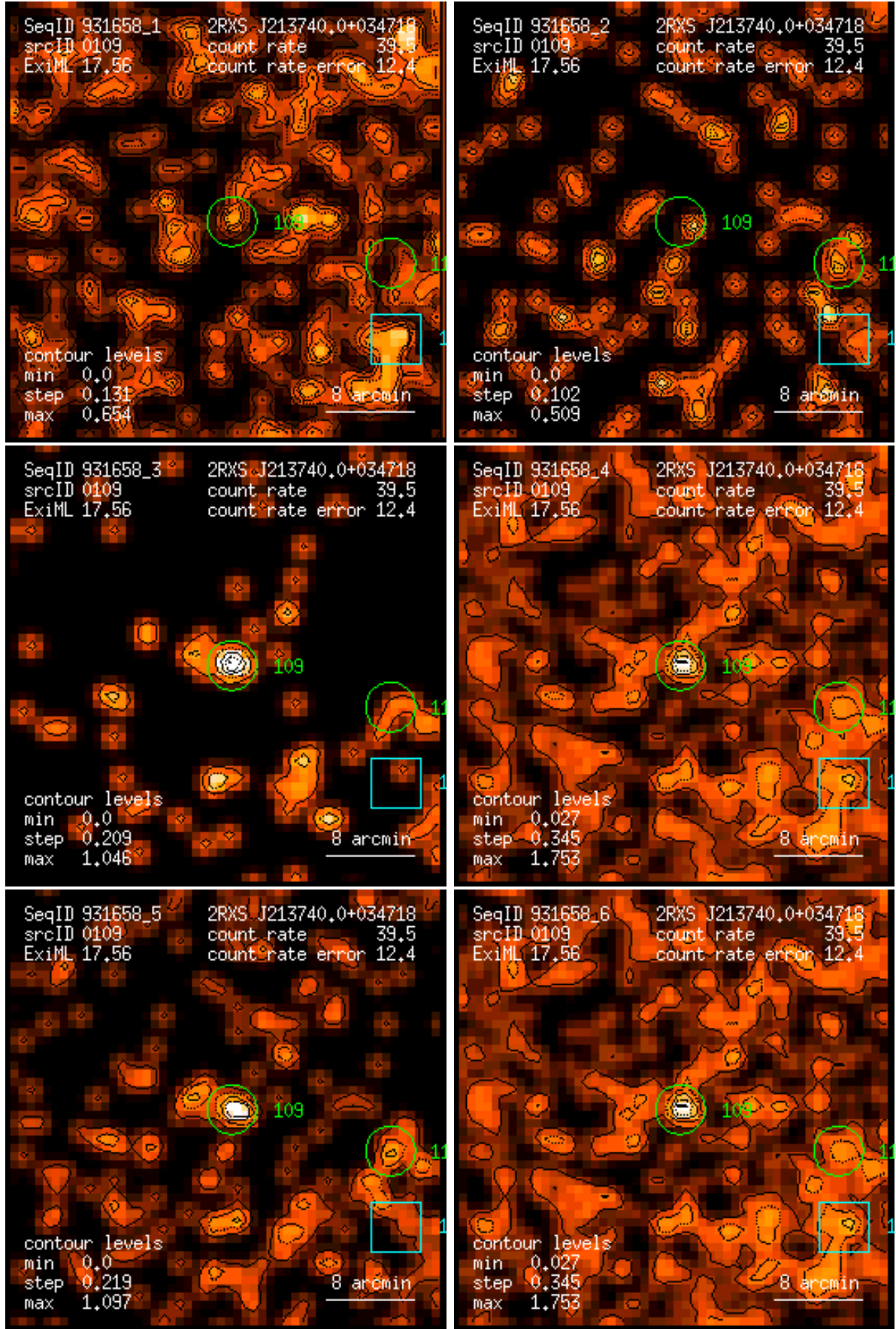
Figure 109: RASS 931658: detection 0109: band rate images, Gaussian filter: (1) PSPC channels 11 – 41, (2) 52 – 90, (3) 91 – 201, (4) 11 – 235, (5) 52 – 201, (6) 11 – 201. Broad band rates in counts/ks. Band rate contour levels in counts/ks/arcmin 2 .
