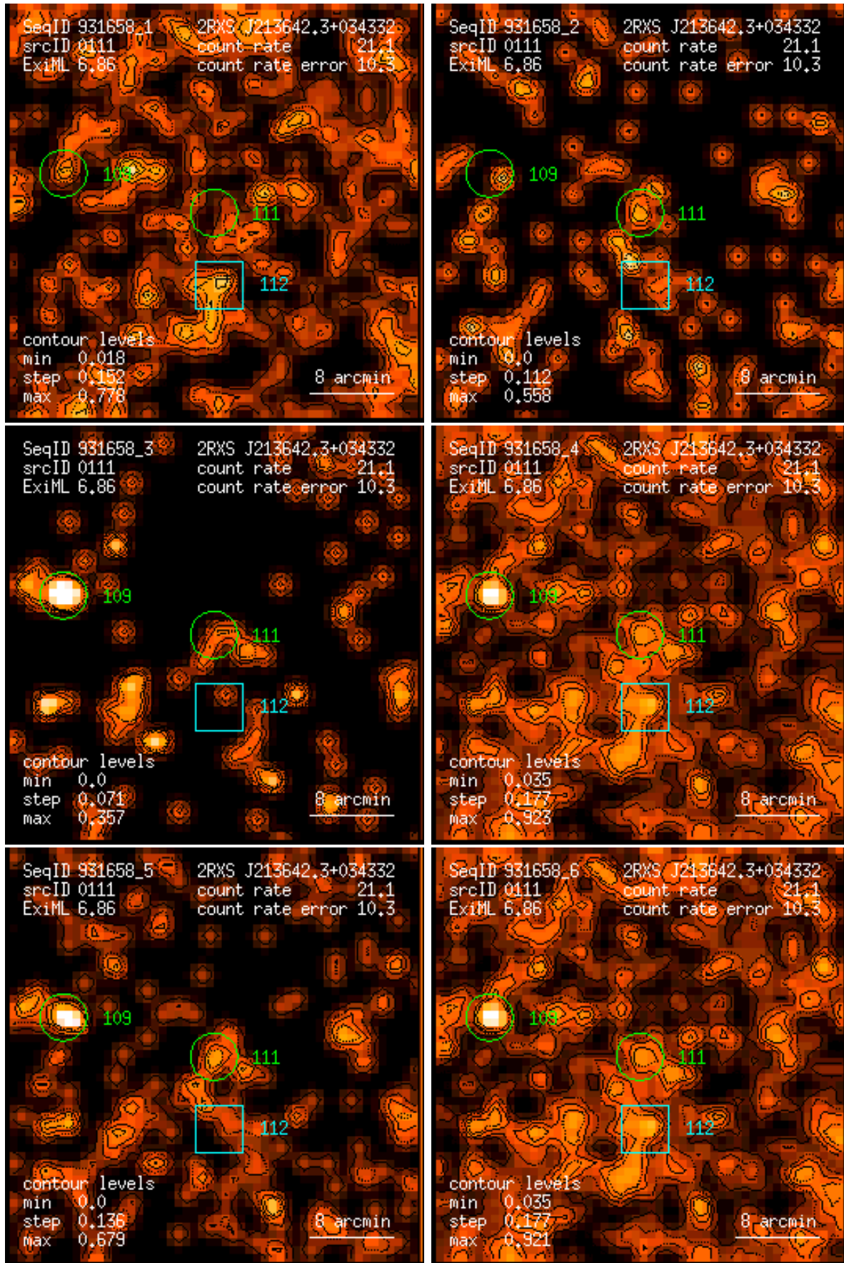
Figure 111: RASS 931658: detection 0111: band rate images, Gaussian filter: (1) PSPC channels 11 – 41, (2) 52 – 90, (3) 91 – 201, (4) 11 – 235, (5) 52 – 201, (6) 11 – 201. Broad band rates in counts/ks. Band rate contour levels in counts/ks/arcmin 2 .
