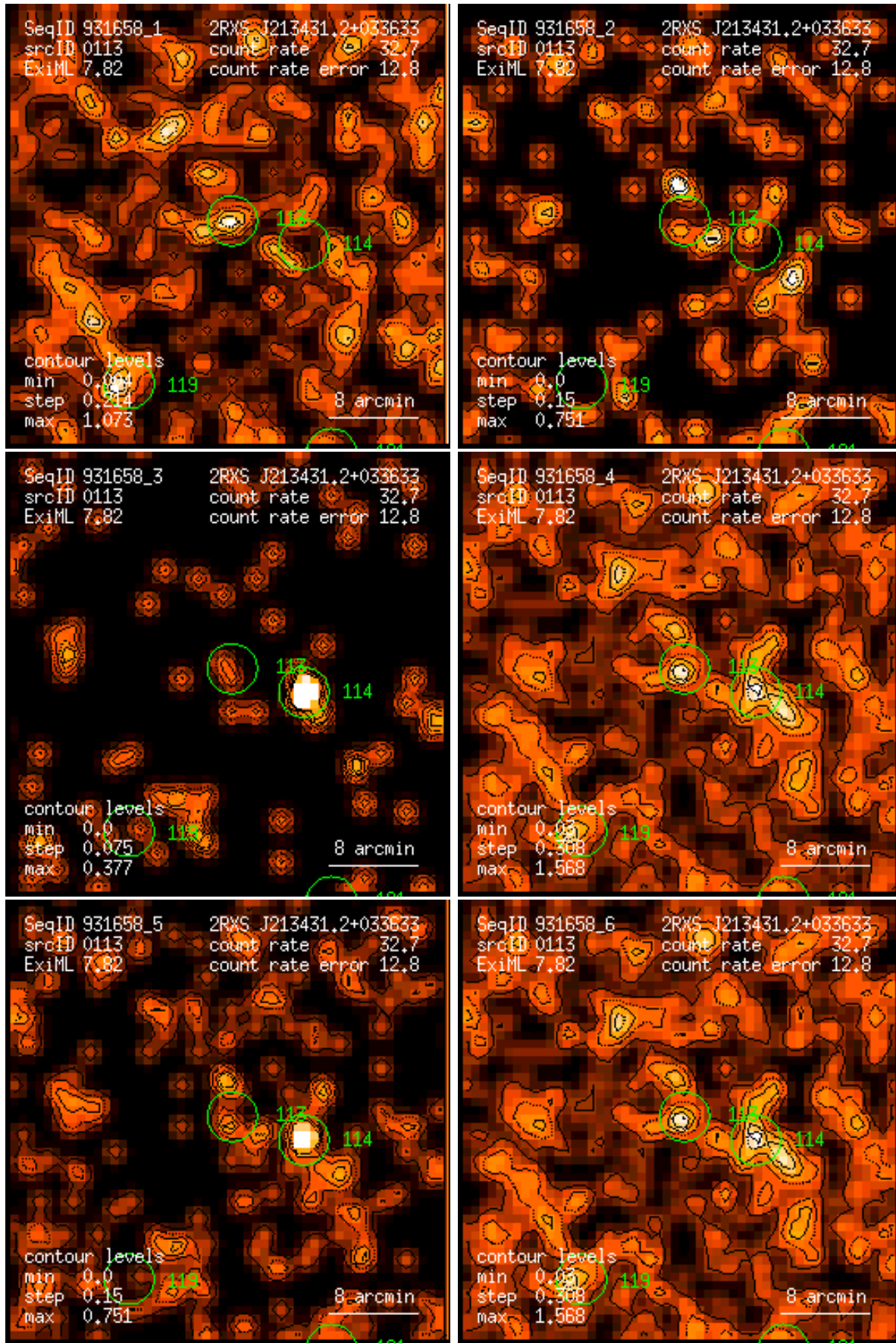
Figure 113: RASS 931658: detection 0113: band rate images, Gaussian filter: (1) PSPC channels 11 – 41, (2) 52 – 90, (3) 91 – 201, (4) 11 – 235, (5) 52 – 201, (6) 11 – 201. Broad band rates in counts/ks. Band rate contour levels in counts/ks/arcmin 2 .
