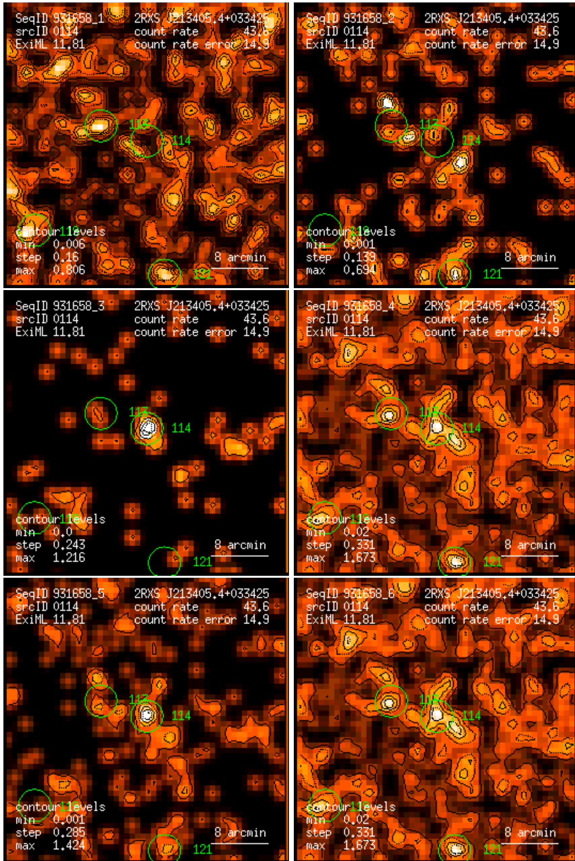
Figure 114: RASS 931658: detection 0114: band rate images, Gaussian filter: (1) PSPC channels 11 – 41, (2) 52 – 90, (3) 91 – 201, (4) 11 – 235, (5) 52 – 201, (6) 11 – 201. Broad band rates in counts/ks. Band rate contour levels in counts/ks/arcmin 2 .
