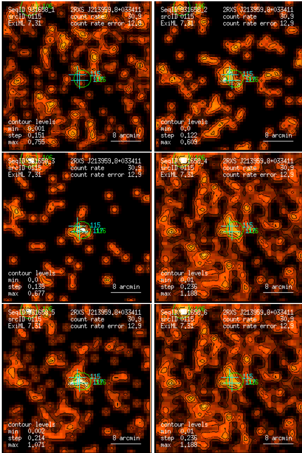
Figure 115: RASS 931658: detection 0115: band rate images, Gaussian filter: (1) PSPC channels 11 – 41, (2) 52 – 90, (3) 91 – 201, (4) 11 – 235, (5) 52 – 201, (6) 11 – 201. Broad band rates in counts/ks. Band rate contour levels in counts/ks/arcmin 2 .
