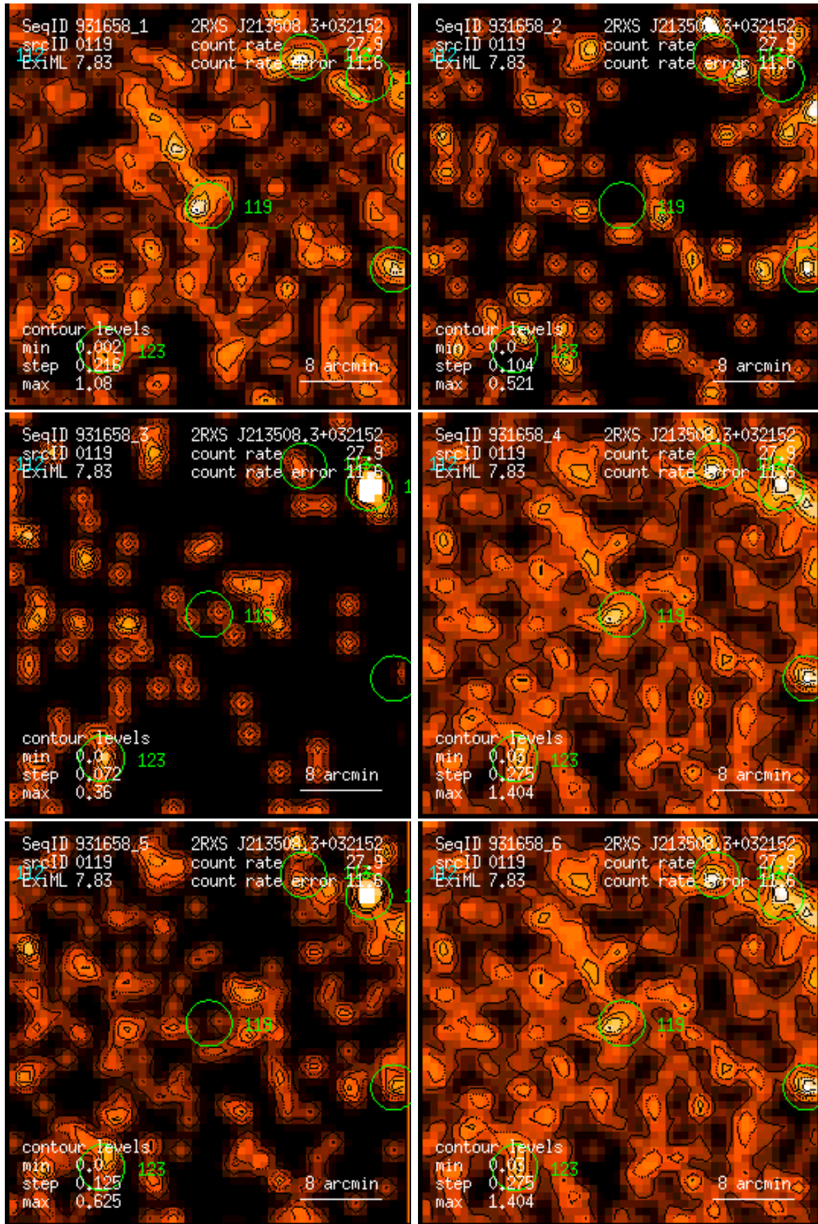
Figure 119: RASS 931658: detection 0119: band rate images, Gaussian filter: (1) PSPC channels 11 – 41, (2) 52 – 90, (3) 91 – 201, (4) 11 – 235, (5) 52 – 201, (6) 11 – 201. Broad band rates in counts/ks. Band rate contour levels in counts/ks/arcmin 2 .
